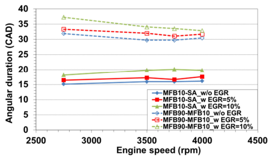
Figure 18: Angular duration as a function of high engine speed at full load and various EGR rates
