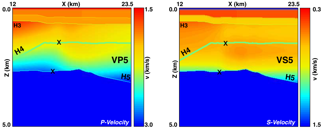
Figure 10: Solution model 2 obtained by tomography with additional constraints on the interface depth at well locations. The RMS value of the traveltimes misfits is 6.0ms. The anisotropy parameters values are: \eta = 8.27\% and \delta = 15.94\% . The crosses represent the wells.
