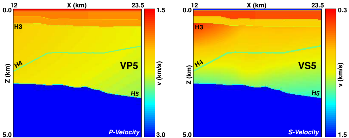
Figure 2: Solution velocity model obtained by tomography. Left: P velocity. Right: S velocity. The RMS value of the traveltimes misfits is 6.2ms . The anisotropy parameters values are: \eta = 6.29\% and \delta = -4.43\% .
