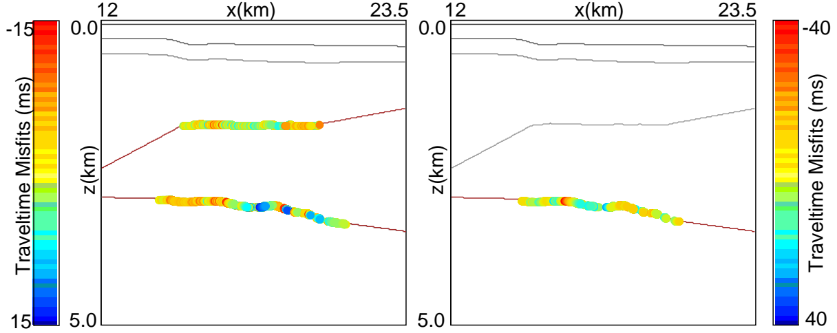
Figure 3: Interfaces of the solution velocity model obtained by tomography and their associated traveltime misfits: impact points of rays reflected on h_4 and h_5 (Left: PP rays. Right: PS rays), colors represent traveltime misfits. Notice that the illuminated zone extends from 14\text{km} to 20.5\text{km} .
