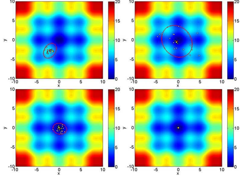
Figure 3: An application of CMA-ES method on the analytical function f(x, y) = \frac{x^2+y^2}{10} - \frac{1}{2} \left( \cos(\frac{2\pi}{5}x) + \cos(\frac{2\pi}{5}y) \right) + 3 . From top left to bottom right, the population at iterations 1, 5, 8 and 20 are represented. The ellipse represents the 95%-isovalue of the Gaussian probability density of the mutation operator with the adaptive covariance matrix.
