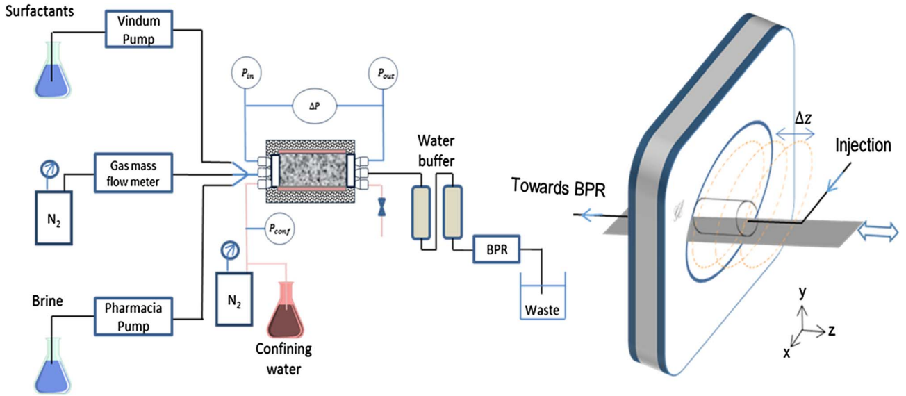
Fig. 2. On the left, the experimental setup to generate foam in the porous medium. On the right, a schematic of the X-ray CT scanner with the core in the gantry.
