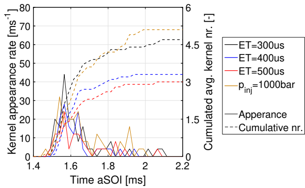
Figure 11: OH* based ensemble-averaged ignition kernel appearance rate and ensemble-averaged cumulated ignition kernels number for a variation of ET and p_{inj} . Conditions: T_{SOI} = 770\text{ K} , \phi_{CH_4} = 0.59 .
