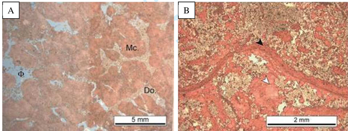
Figure 7. Transmitted light plane-polarized photomicrographs of A) Family F1 sample showing macropores ( \Phi ), calcite mesoclots (Mc.) and dolomite cement (Do.) and B) Family F2 sample showing dolomitized matrix, syntaxial cement (white arrow) and fabric-preserving replacement of aragonitic allochems (black arrow).
