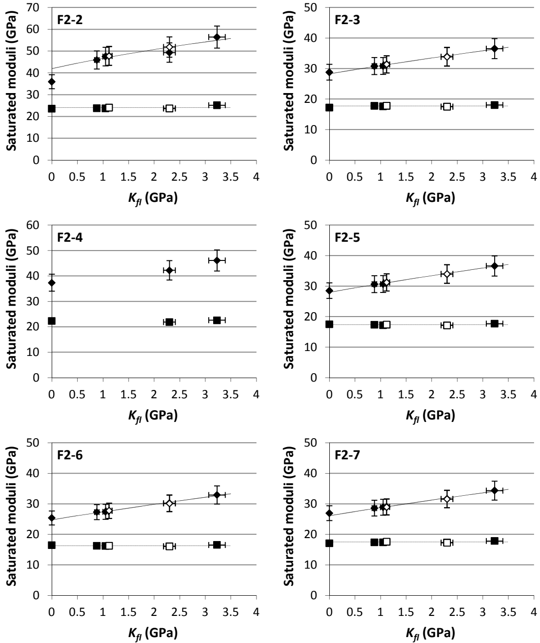
Figure 11. Petroacoustic signature of fluid substitution for F2 samples. Same captions as in Figure 10.
