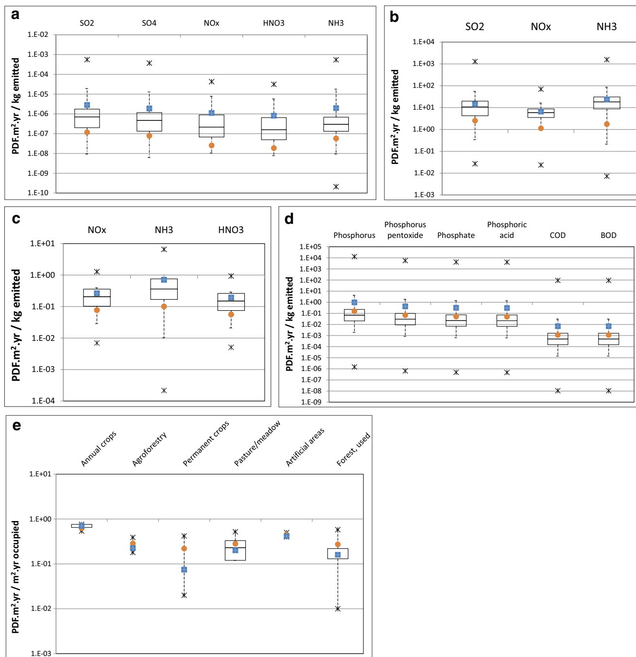
Fig. 5 Spatial variability of impact indicators contributing to the ecosystem quality AoP. a Freshwater acidification. b Terrestrial acidification. c Marine eutrophication. d Freshwater eutrophication. e Land occupation on ecosystem quality
