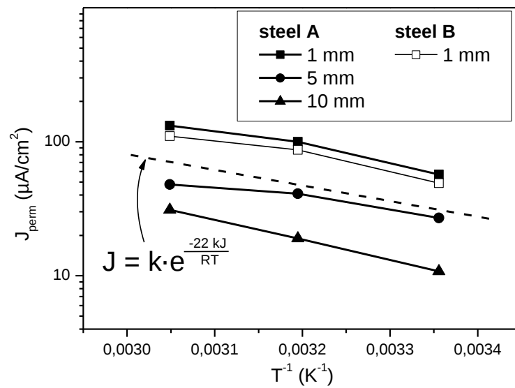
Figure 14: Evolution of the steady-state permeation flux with temperature, for different experiments at pH 3.5 under 10 % H 2 S and 90 % CO 2 .
