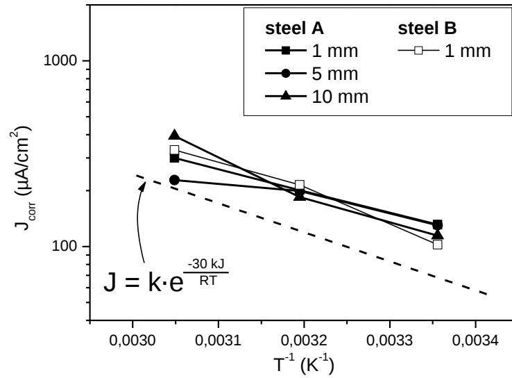
Figure 15: Evolution of the corrosion current with temperature, for different experiments at pH 3.5 under 10 % H_2S and 90 % CO_2 .
