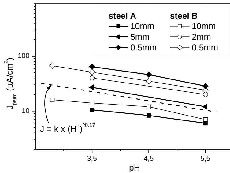
Figure 10: Evolution of the steady-state permeation flux with pH for experiments under 100 mbar \text{H}_2\text{S} and 900 mbar \text{CO}_2 , for different steel grades and different membrane thicknesses.
