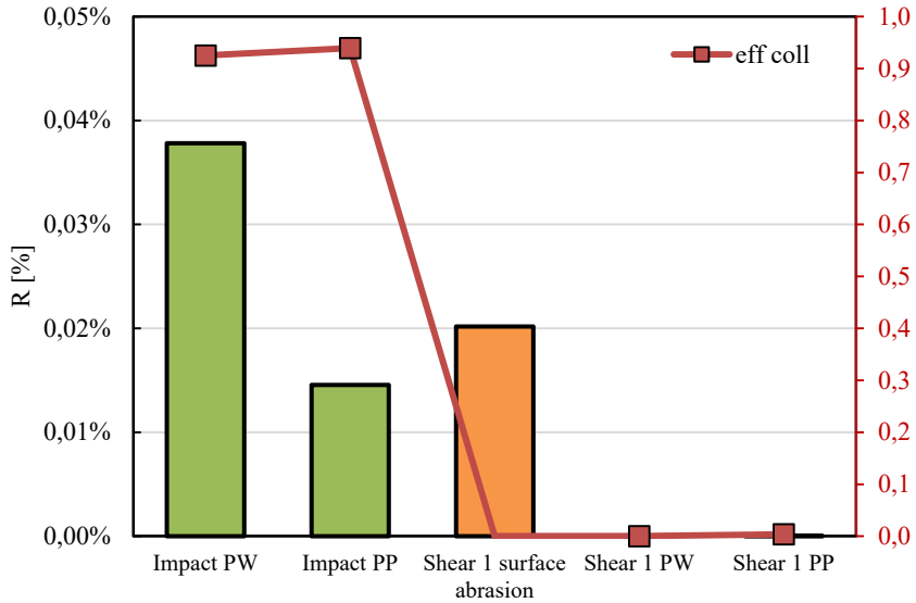
Figure 21. Extents of breakage, R, and collision efficiency factor, \eta_c , of the regions "Impact" (in green) and "Shear 1" (in orange) as a result of surface abrasion, particle-wall and particle-particle collisions
