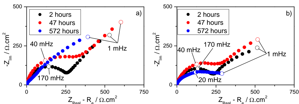
Figure 3: Typical impedance of pure iron in 35 g/L NaCl solution saturated with 100 kPa \text{H}_2\text{S} at various exposure times, without (a) and with (b) \text{O}_2 pollution.
