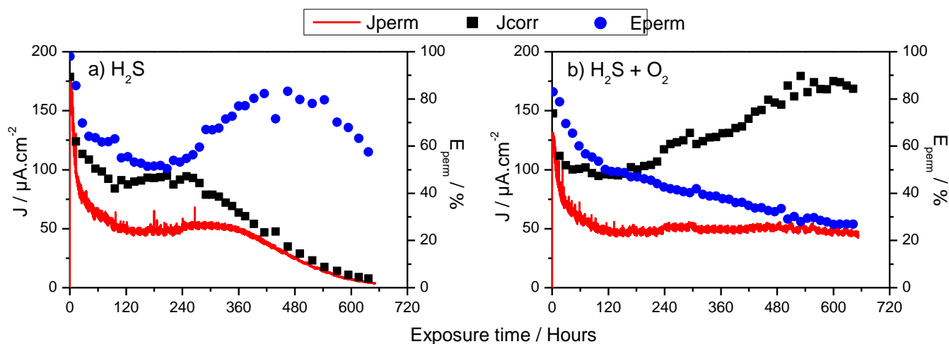
Figure 9 : Time evolution of corrosion current densities, hydrogen permeation current densities, and permeation efficiency ( E_{\text{perm}} ) for the tests on X65 in NACE A solution, without (a) and with (b) O 2 pollution.
