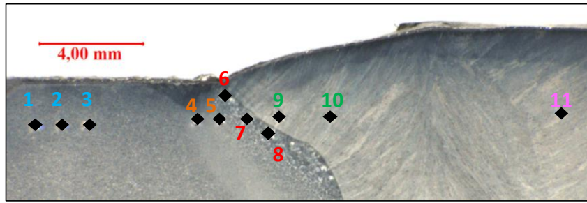
Figure A1: “1.5 mm under top skin” line
