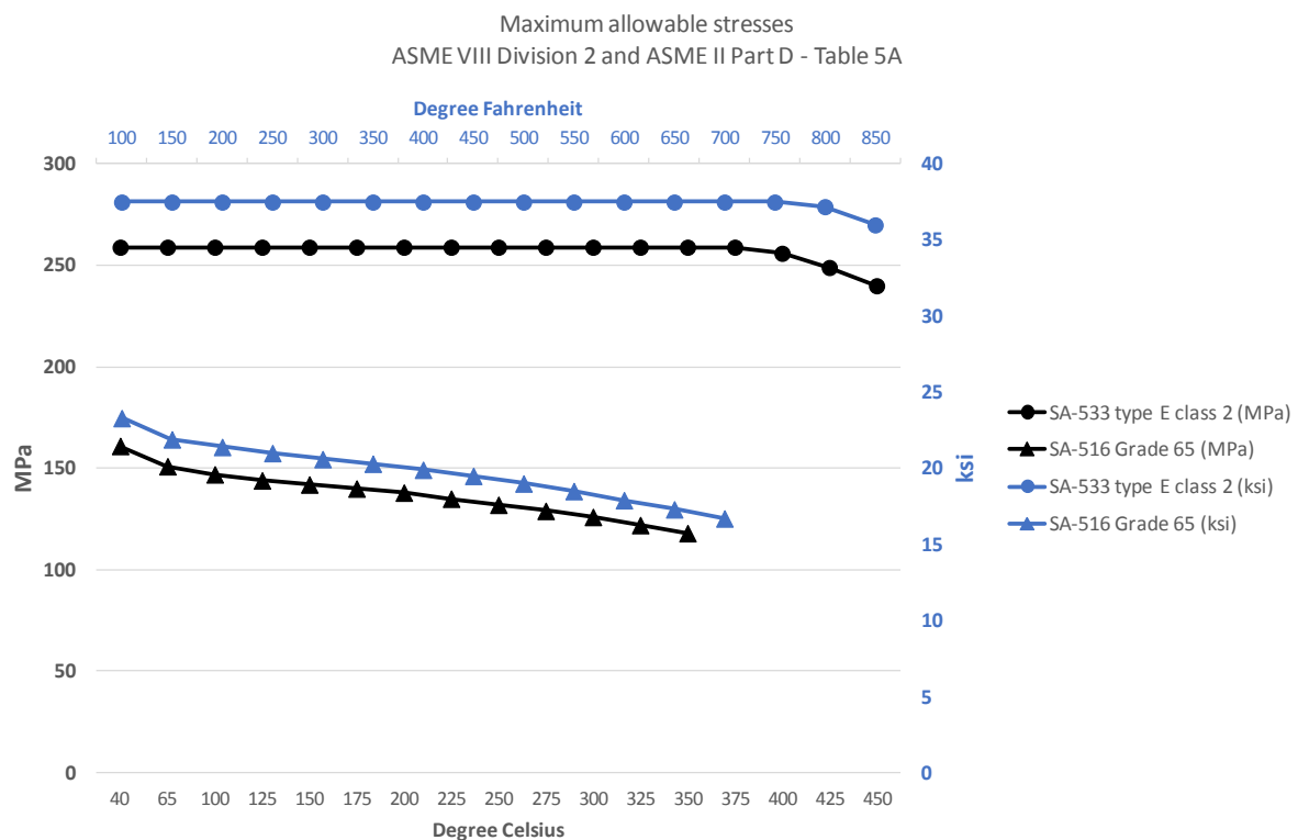
Figure 2 : higher maximum allowable stresses are provided by SA-533 type E class 2
