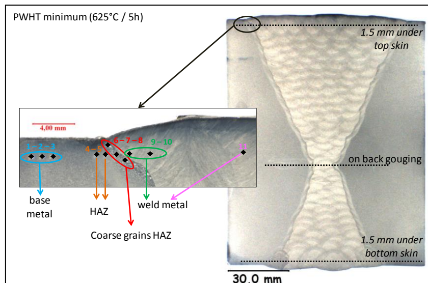
Figure 5 - 120 mm thick Submerged Arc Welding (SAW) cross section macrograph
