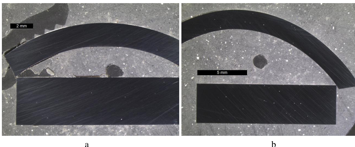
Figure 10 : Cross section of Ubend and 4 points bend samples a: SA-516 Gr65 ; b : SuperElso ® 533E
