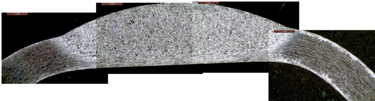
Figure 14: Cross section of weld on U-bend on Duplex 2205
