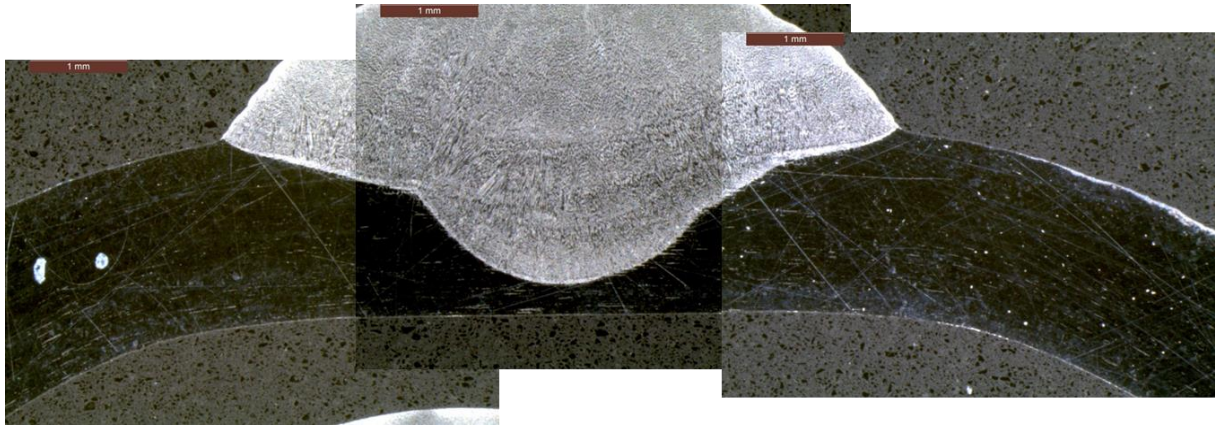
Figure 13: Cross section of weld on U-bend on SS316L
