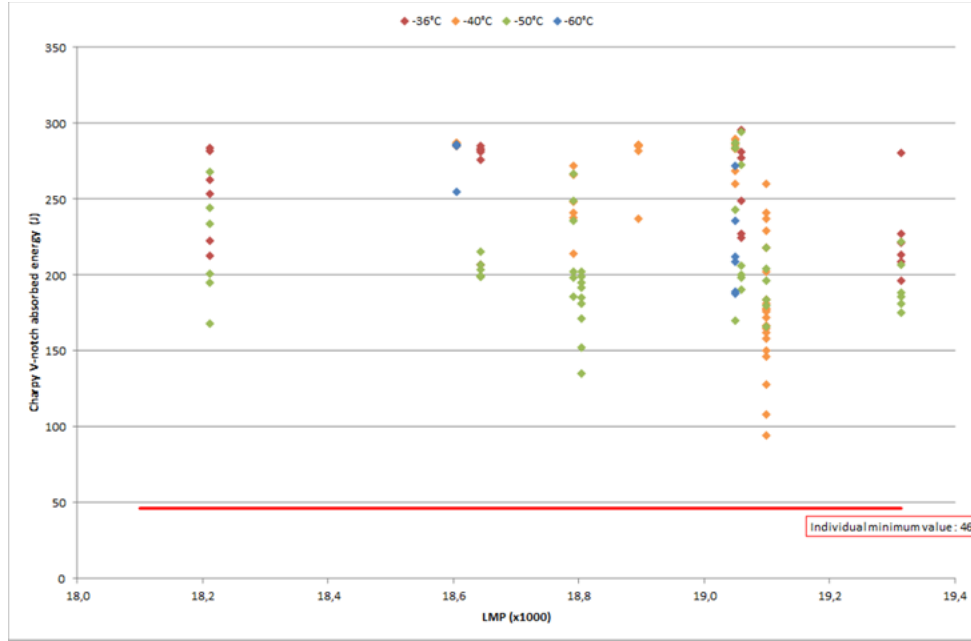
Figure 3 : Charpy-V notch impact toughness depending on LMP (quarter-thickness)
