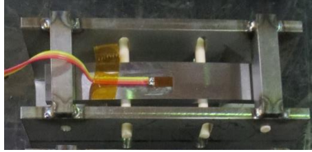
Figure 6: 4 point bend device with strain gauge used during the pre-deformation
