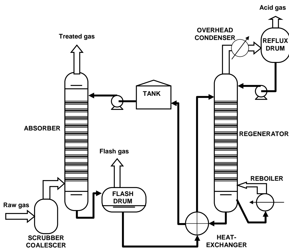
Figure 1 A schematic amine process flow diagram
