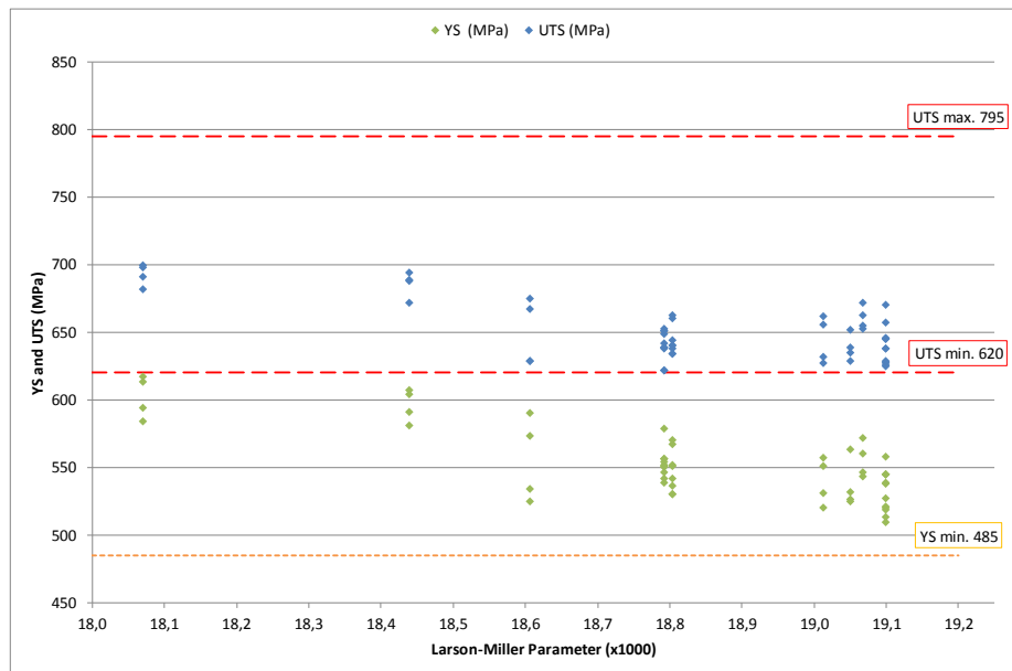
Figure 4 : Transverse yield strength and tensile strength depending on LMP
