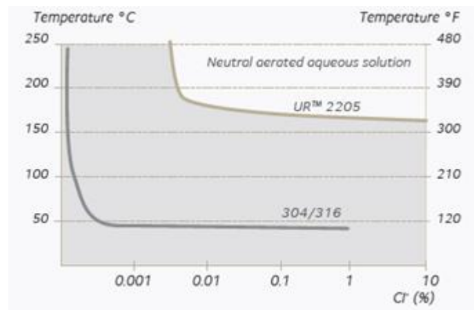
Figure 11: Typical domains of resistance to stress corrosion cracking of austenitic grades and 2205 duplex grade
