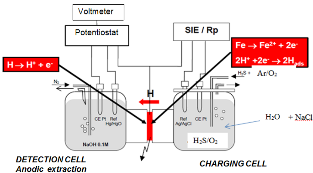
Figure 2 : Permeation set up
