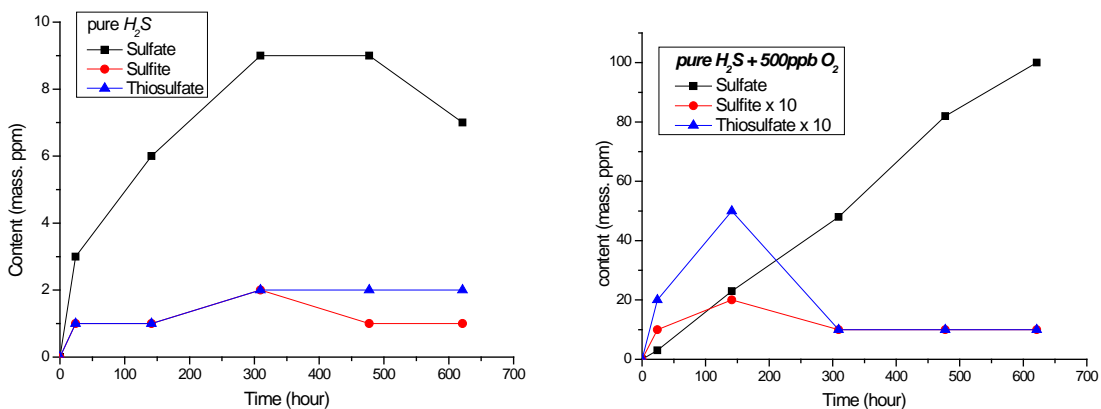
Figure 5 : S-O content in test media
