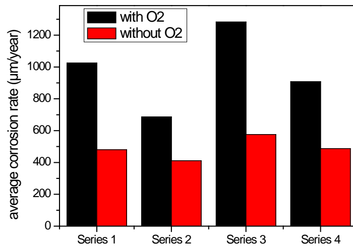
Figure 6 : Comparisons of corrosion rates for several tests with and without oxygen pollution
