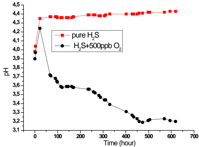
Figure 4 : pH trend of tests solutions
