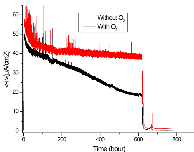
Figure 8 : Permeation curves in H 2 S medium with or without oxygen.
