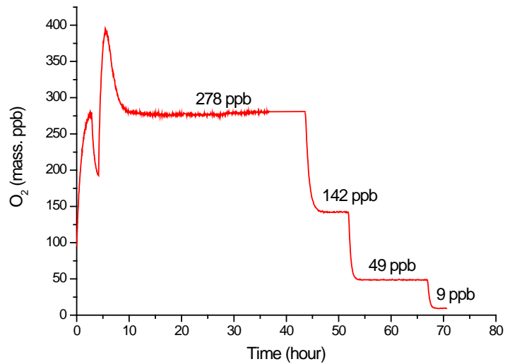
Figure 3 : Control of oxygen content in the test medium
