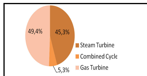
Figure 2: Existing generation capacity profile in Saudi Arabia
