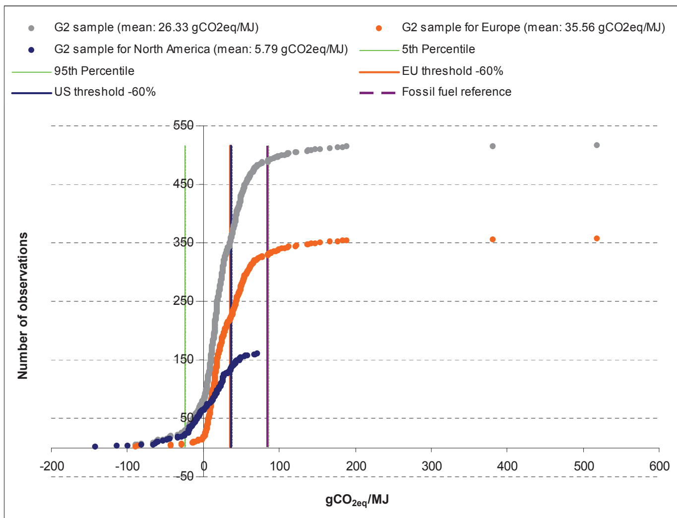
Figure 4 - Dispersion of LCA GHG emission results included in the database for G2 biofuels and for the different geographical location
