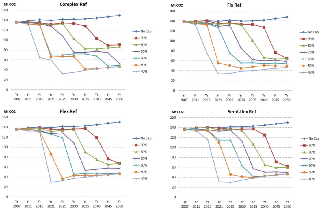
Figure 16: Fossil CO_2 emissions of transport for the various models
