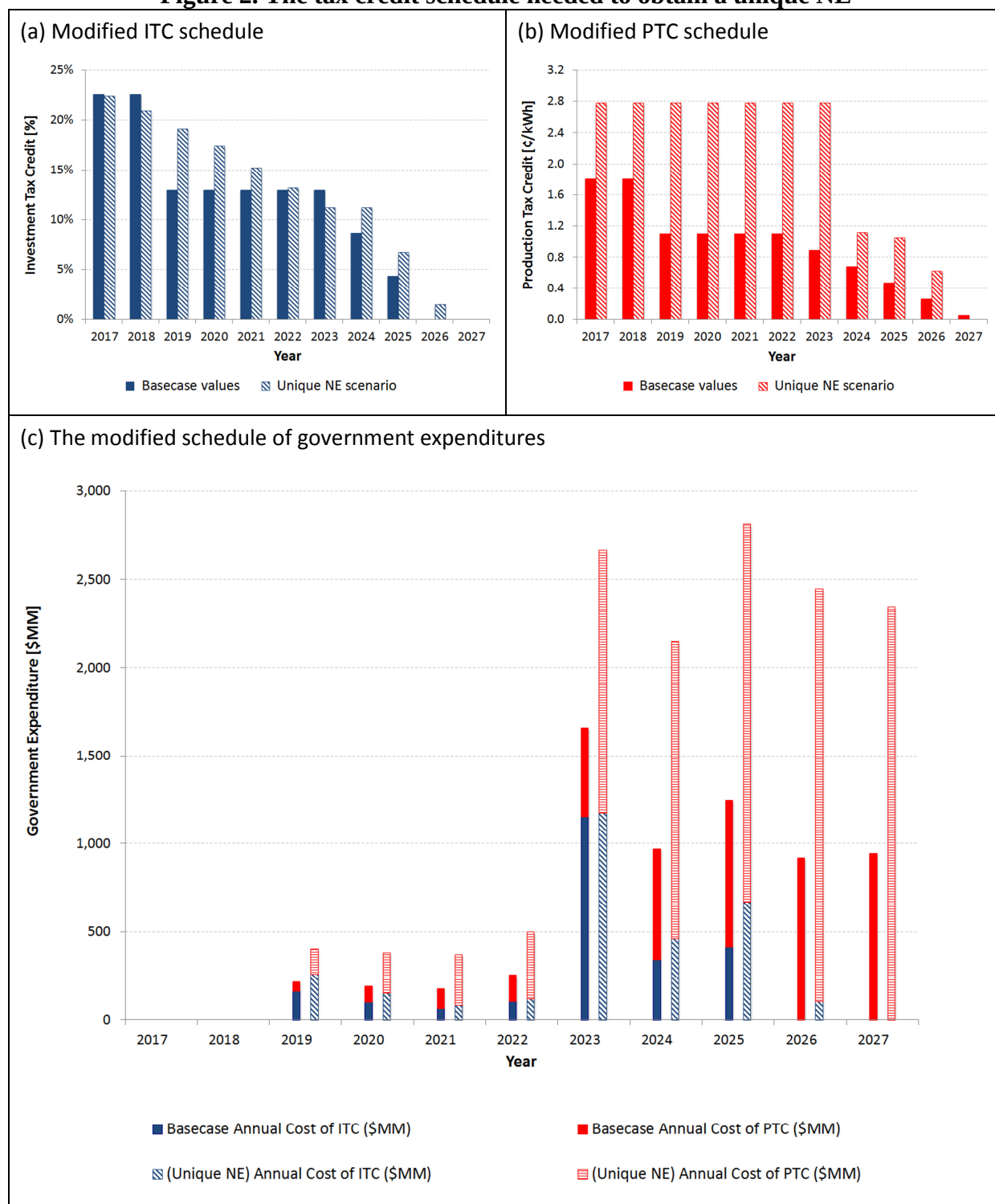
Figure 2. The tax credit schedule needed to obtain a unique NE
