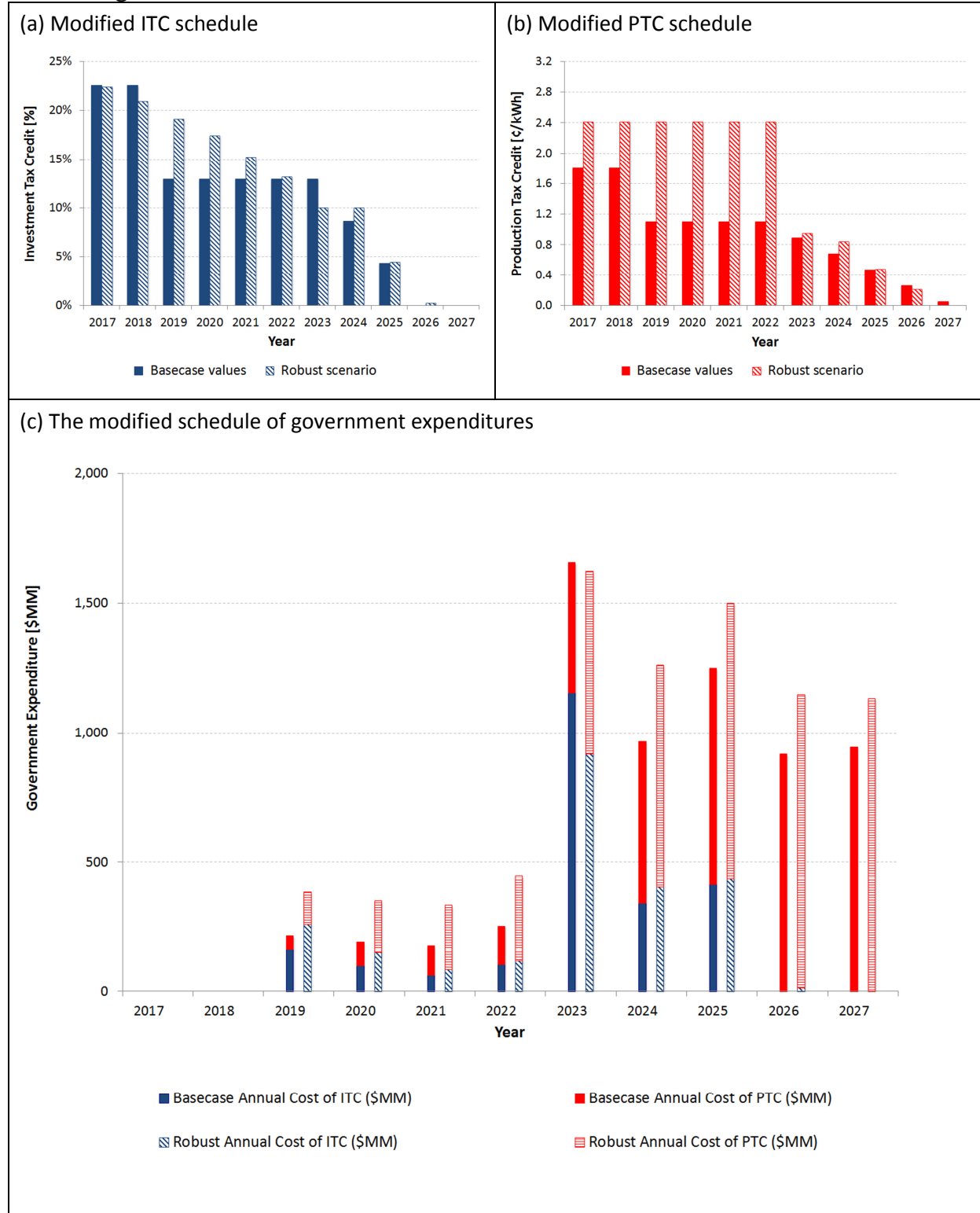
Figure 1. The modified ACCD tax credits schedule under a robust scenario
