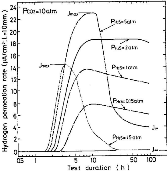
Figure 4 : Hydrogen permeation rate through 10 mm thick API X70 steel membranes in synthetic seawater and at different H_2S partial pressure [34].
