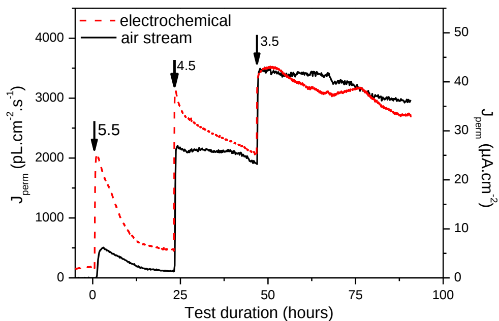
Figure 6: permeation transients measured simultaneously by air stream technique and electrochemical method, for two identical membranes (0.5 mm) of steel B exposed to test solution saturated with 1 bar H 2 S, and with successive pH steps. Electrochemical membrane with Pd coating on the exit face.
