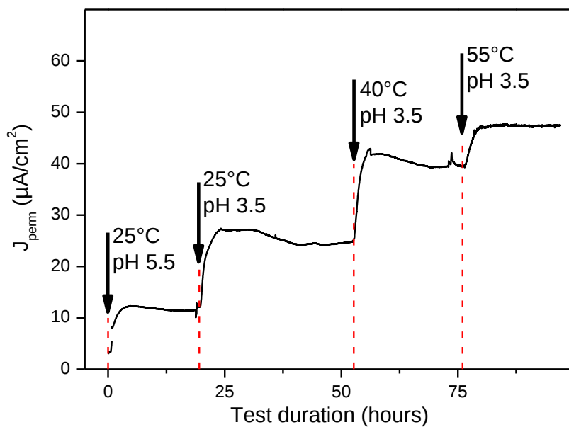
Figure 14: Impact of temperature on permeation transient measured for a 5 mm membrane of steel A exposed to test solution at various pH and under 100 mbar H_2S and 900 mbar CO_2 .
