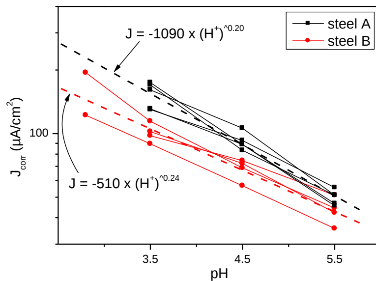
Figure 13: Evolution of the corrosion current density evaluated from R_p measurements as a function of pH and for experiments under 100 mbar H_2S and 900 mbar CO_2 , for different steel grades.
