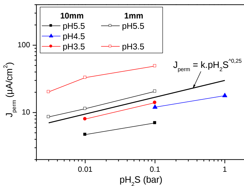
Figure 10: Evolution of the permeation flux with H_2S partial pressure ( CO_2 balance to 1 bar) for different pH and membrane thicknesses (steel B).
