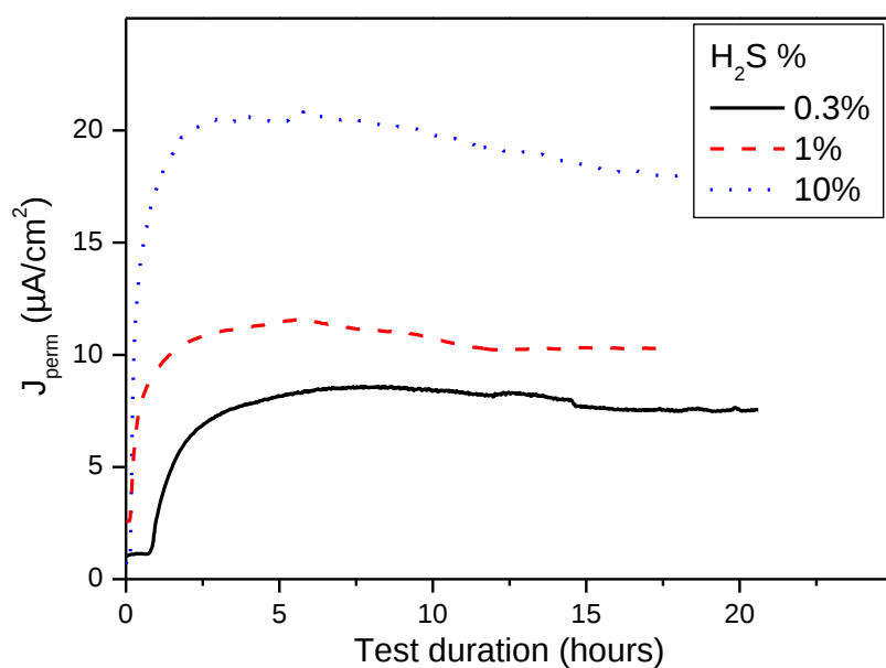
Figure 8: Permeation transients measured for 1 mm membranes of steel A exposed to test solution at pH 3.5 saturated under 1 bar with different H_2S / CO_2 ratios.
