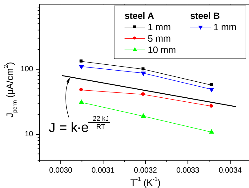
Figure 15: Evolution of the permeation flux with temperature, for different experiments at pH 3.5 under 10 % \text{H}_2\text{S} and 90 % \text{CO}_2 .
