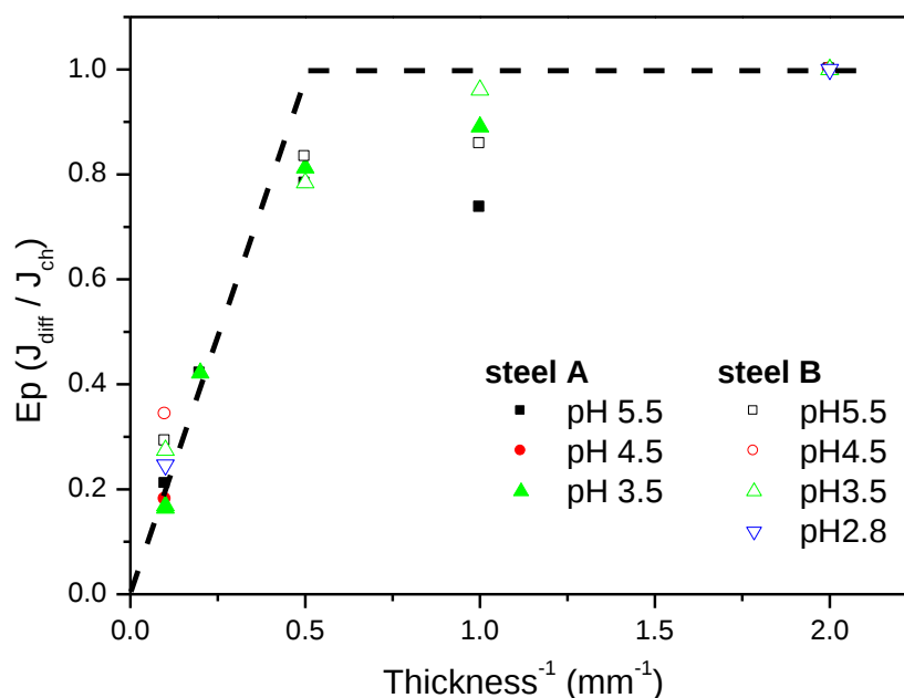
Figure 19: Evolution of permeation efficiency ( E_p = J_{diff} / J_{ch} ) with membrane thickness, for all experiments under 100 mbar H_2S and 900 mbar CO_2 .
