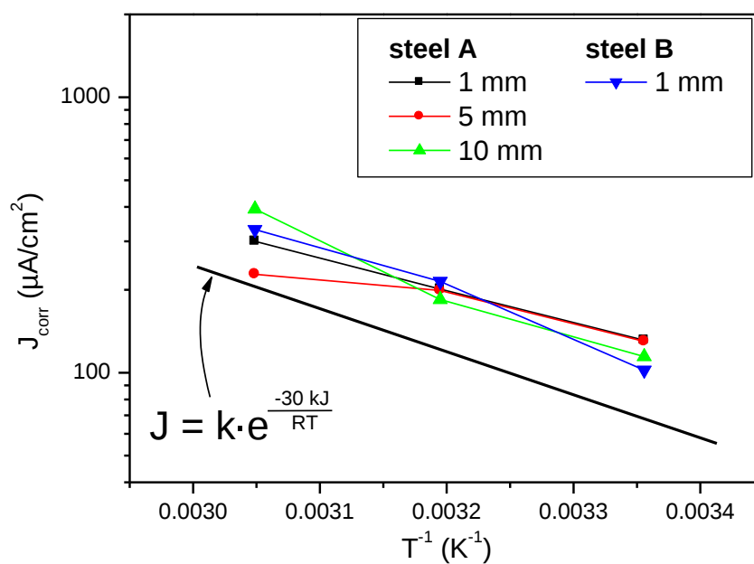
Figure 16: Evolution of the corrosion current with temperature, for different experiments at pH 3.5 under 10 % \text{H}_2\text{S} and 90 % \text{CO}_2 .
