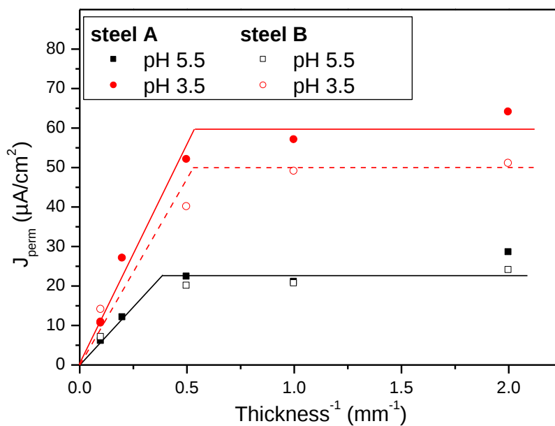
Figure 18: Evolution of permeation flux with membrane thickness for different experiments under 100 mbar H_2S and 900 mbar CO_2 .
