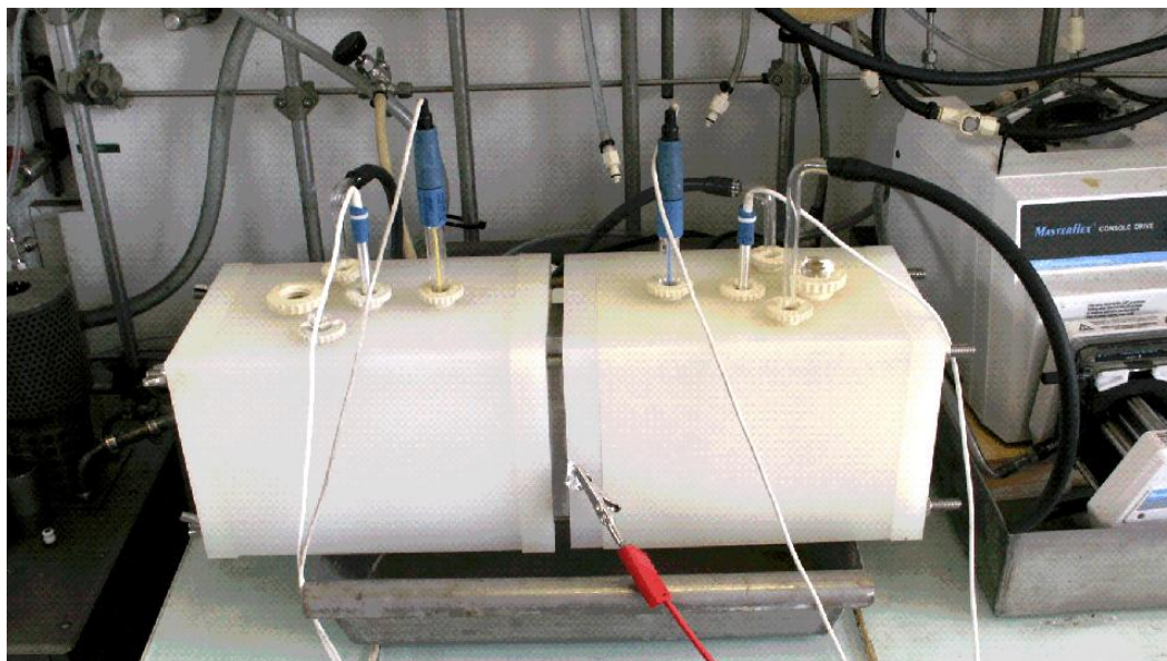
Figure 5: Devanathan-Stachurski cell for permeation measurements on thick specimens.
