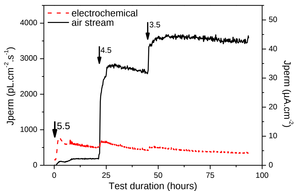
Figure 7: permeation transients measured simultaneously by air stream technique and electrochemical method, for two identical membranes (0.5 mm) of steel B exposed to test solution saturated with 1 bar H_2S , and with successive pH steps. Electrochemical membrane without Pd coating on the exit face.
