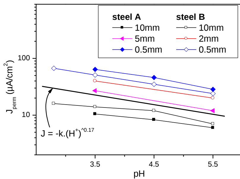
Figure 11: Evolution of the permeation flux with pH for experiments under 100 mbar \text{H}_2\text{S} and 900 mbar \text{CO}_2 , for different steel grades and different membrane thicknesses.
