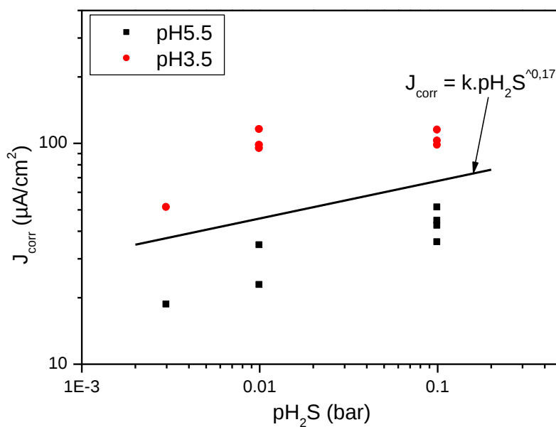
Figure 12: Evolution of the corrosion current density evaluated from R_p measurements as a function of \text{H}_2\text{S} partial pressure ( \text{CO}_2 balance to 1 bar) and for different test solution pH (steel B).
