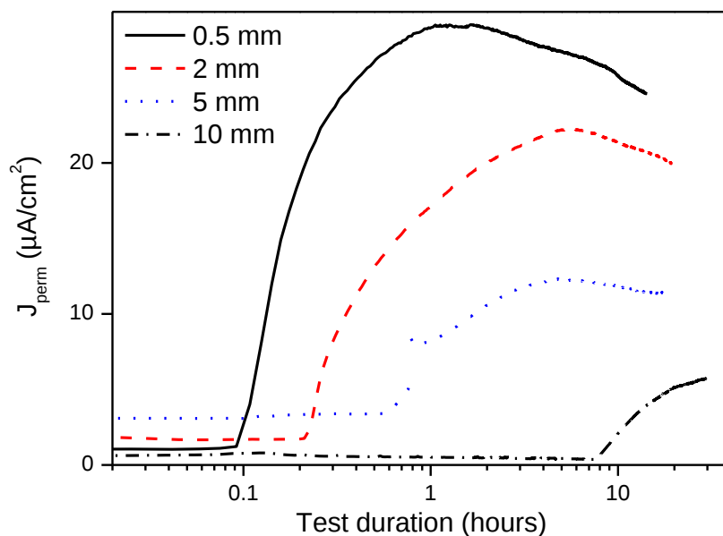
Figure 17: Permeation transients measured for steel A membranes of different thickness, exposed to test solution at pH 5.5 saturated with 100 mbar H_2S and 900 mbar CO_2 .
