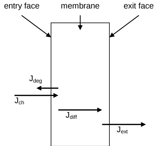
Figure 1: Different hydrogen fluxes through a steel membrane.
