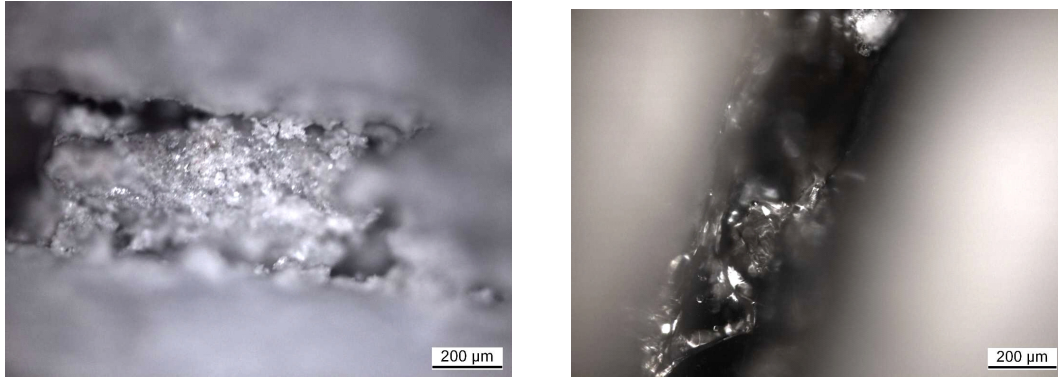
Figure 16 – Films deposited in a scratched coating area immersed in a solution of NaCl-1 % under cathodic polarisation ( -0.85 V_{/Ag/AgCl} ) during 40 hours: 20°C (left) ; 60°C (right).
