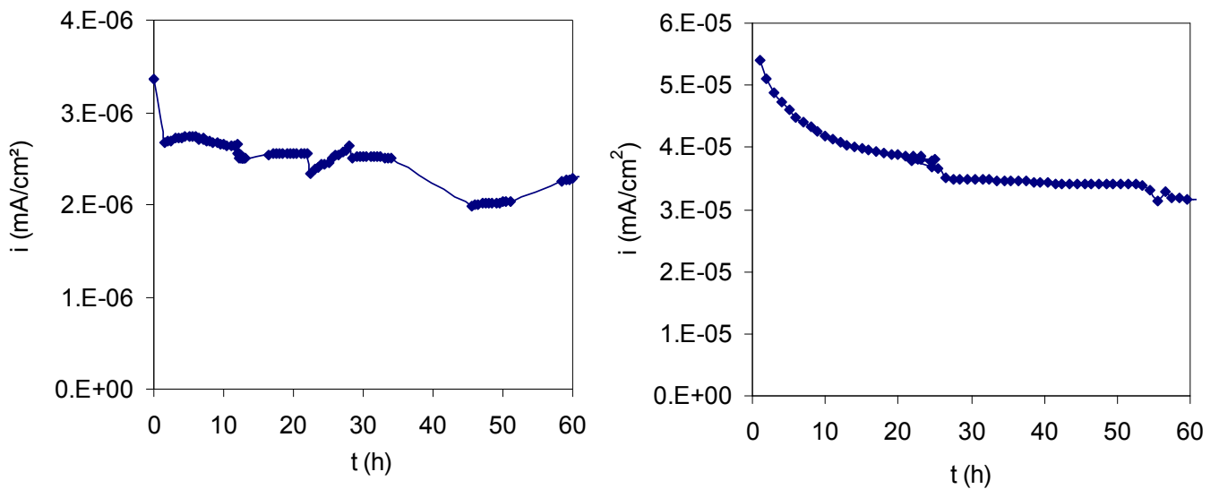
Figure 12 – Variation in current density (with respect to total exposed area) with the progress of film deposition at 20°C on bare steel panels under cathodic polarisation : -0.85 V_{/Ag/AgCl} (left); -1.1 V_{/Ag/AgCl} (right).
