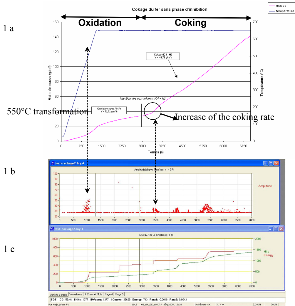
Figure 1: TGA and AE measurements on an oxidised iron surface
