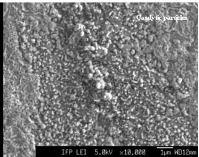
Figure 6: SEM picture of the reduced iron surface after 5 hours of reduction at 650^\circ\text{C} and 300 seconds of coking at 650^\circ\text{C}
