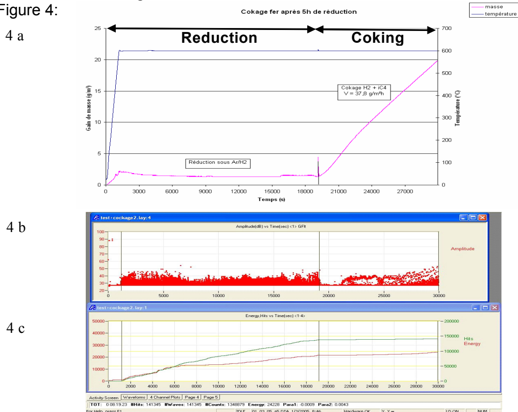
Figure 4: TGA and AE measurements on a reduced iron surface
