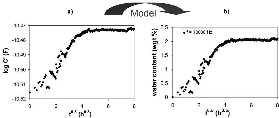
Figure 2 : Water uptake monitoring by EIS in the pure epoxy-amine polymer at 100°C; a) capacitance evolution with square root of time; b) water content given by EIS according to Brasher and Kinksbury law [3].
