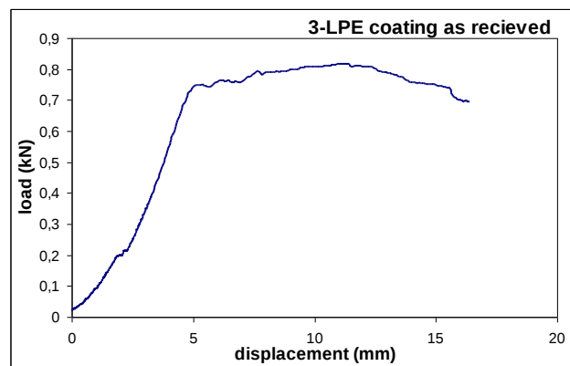
Figure 5 - Peeling of the B-3LPE coating as received
