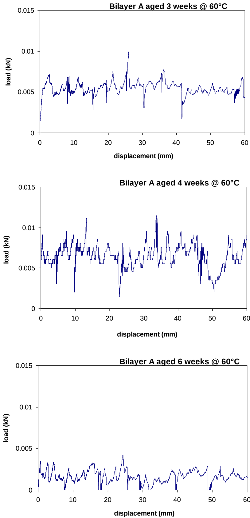
Figure 8 - Peeling of A-bi-layer coating exposed to 95 % relative humidity at 60°C: results after 3, 4 and 6 weeks
