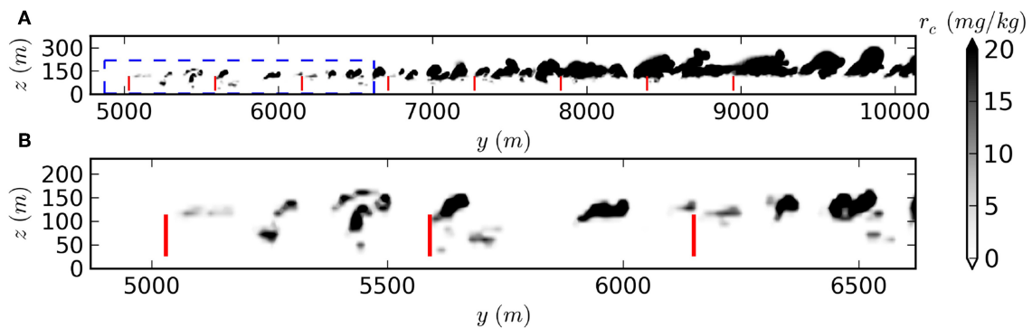
FIGURE 11 | Vertical cross-section of the cloud mixing ratio through the whole fourth row of the wind farm (A) and the firsts wind turbines (B) . The red plain lines (–) indicate the locations of wind turbines. The blue dashed line (–) in A indicates the area of B.
