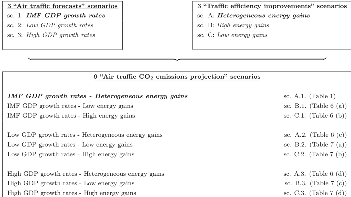
Figure 2: The nine “Air traffic CO 2 emissions projection” scenarios.
