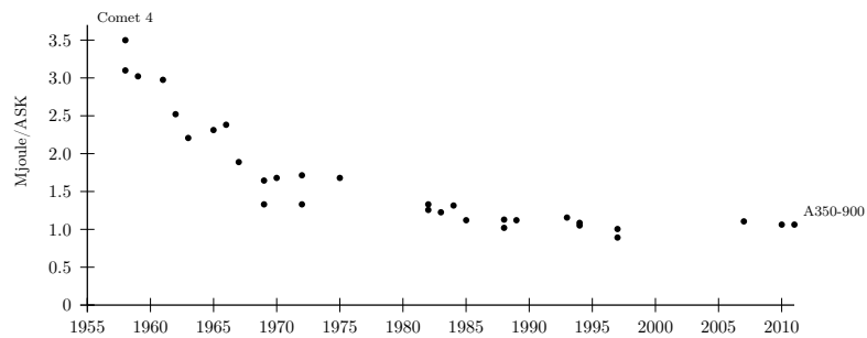
Figure 3.1: Evolution of average Jet-Fuel consumption by aircraft vintage expressed in Mjoule per ASK (1955-2010).
