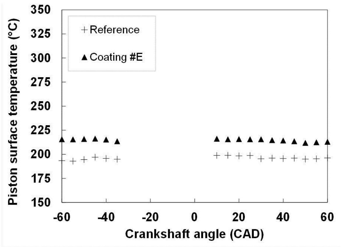
Figure 2S. Piston surface temperatures at 2000 rpm, 4 bar IMEP ( \lambda = 1.21 ) at the end of exhaust stroke (from -60 to 0 CAD) and beginning of intake stroke (from 0 to 60 CAD).
