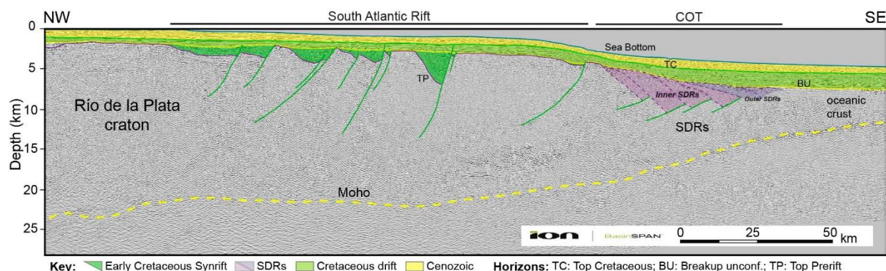
Fig. 14: Depth-converted dip seismic section of the northern Argentinean margin (southern Salado basin), between the Tandilia and Salado FZs. Location in Fig. 16.
