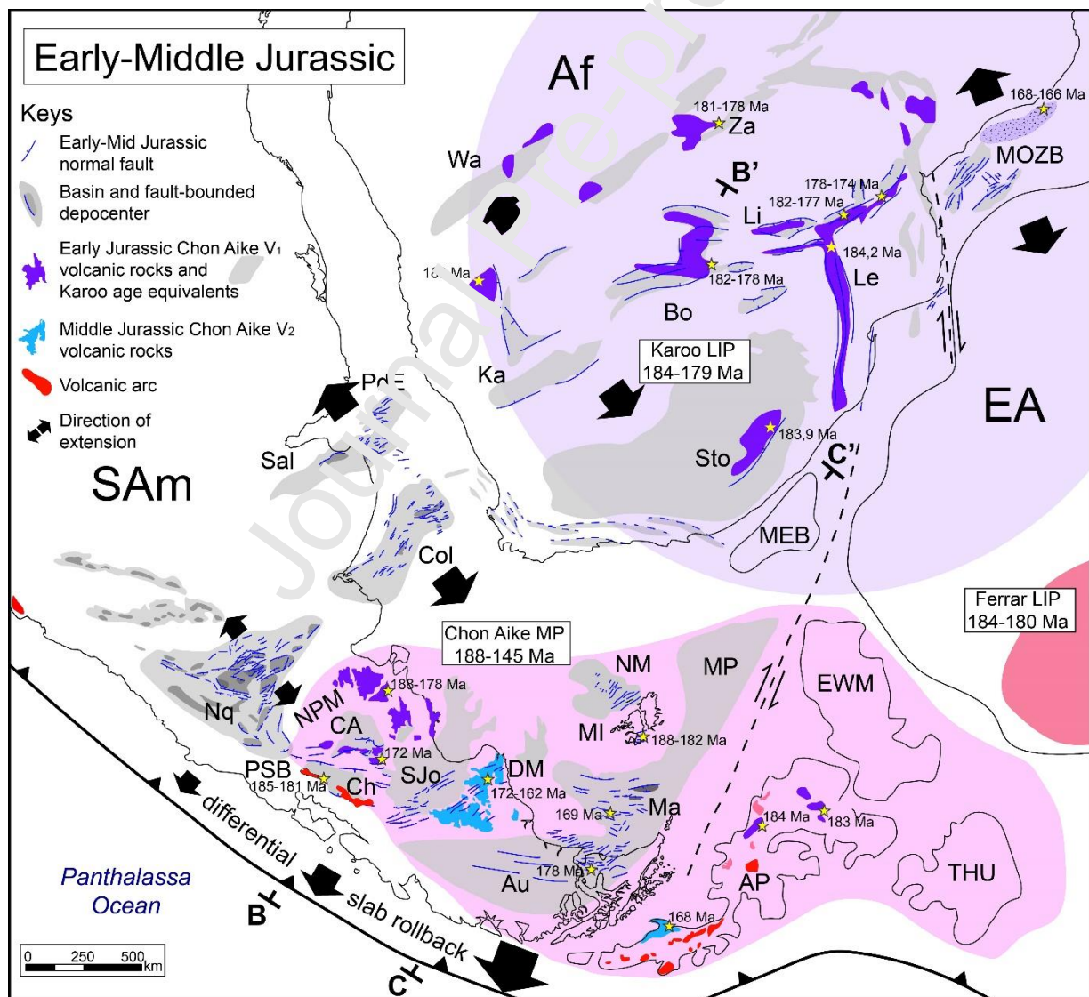
Fig. 10: Paleo-tectonic reconstruction of SW Gondwana in the Early-Mid Jurassic. Gondwana fit after Dalziel et al. (2013). Eastern Africa and Eastern Antarctica are impacted by the Karoo
