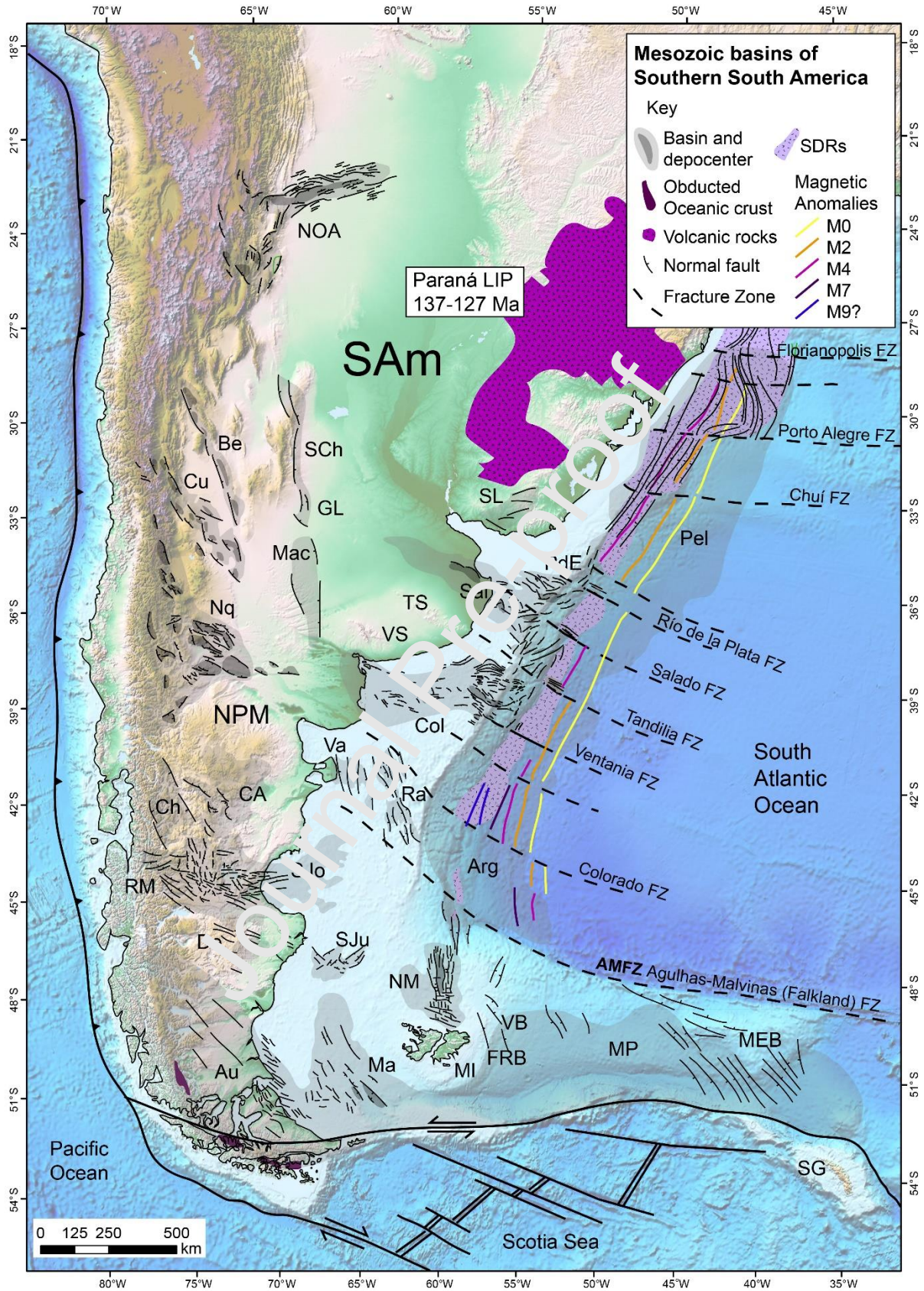
Fig. 3: Map of the main Mesozoic basins of SE South America (SAm). NOA: Northwest Argentina Cretaceous basin, SCh: Sierras Chicas, GL: General Levalle, Mac: Macachín, Be: Bermejo, Cu: Cuyo basin, Nq: Neuquén, NPM: North Patagonian Massif, CA: Cañadón
