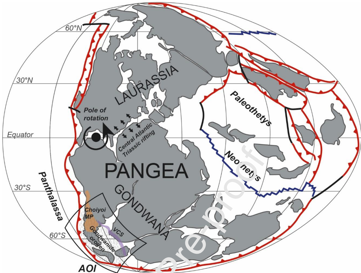
Fig. 7: Paleo-tectonic map of the Pangea supercontinent at the end of the Paleozoic (circa 250 Ma) after Riel et al. (2018). Euler rotation pole of Pangea from Torsvik et al. (2012). Note the location of the Area of Interest (AOI), the Gondwanide orogen, the Choiyoi Magmatic Province and the Ventania-Cape foldbelt (VCS).
