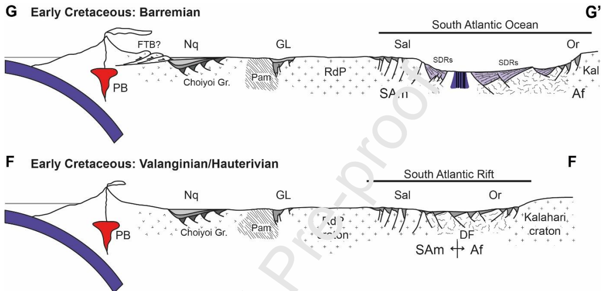
Fig. 17: Schematic cross sections of the SW Gondwana margin. F-F' is a transect for the Valanginian, with a magmatic arc represented by the Patagonian Batholith. The General Levalle graben (GL) is depicted (after Webster et al., 2004). Rifting in the South Atlantic Rift area (Fig. 15a) across the southern Salado basin (Fig. 14) and the Orange basin. Transect G-G' represents the same section in the Barremian, with SDRs emplacement along this segment in the Hauterivian, and breakup near the Hauterivian/Barremian boundary. Compression is interpreted for the Neuquén basin retroarc (Nq), possibly with development of a fold and thrust belt (FTB). See approximate location in the map in Fig. 15 and 16.
