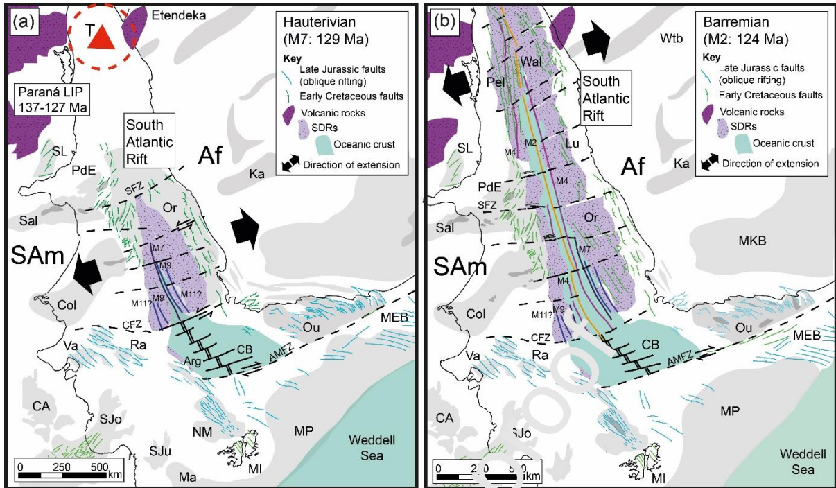
Fig. 15: Paleo-tectonic reconstructions of the South Atlantic Rift in the Early Cretaceous: a) Hauterivian: the southernmost Rawson/Valdés - Outeniqua segment where breakup occurred in the Valanginian is in the drift phase; north of the Colorado fracture zone (CFZ), SDRs are being emplaced along different segments during the breakup process. The South Atlantic rift has an approximate width of 500 km. Further North in the Pelotas/Walvis segment, the Paraná-Etendeka basalts are produced by the Tristan da Cunha (T) hotspot before onset of rifting; b) Barremian: active rifting in the Pelotas/Walvis segment, while south the Salado fracture zone (SFZ) the conjugate margins are in the drift phase.
