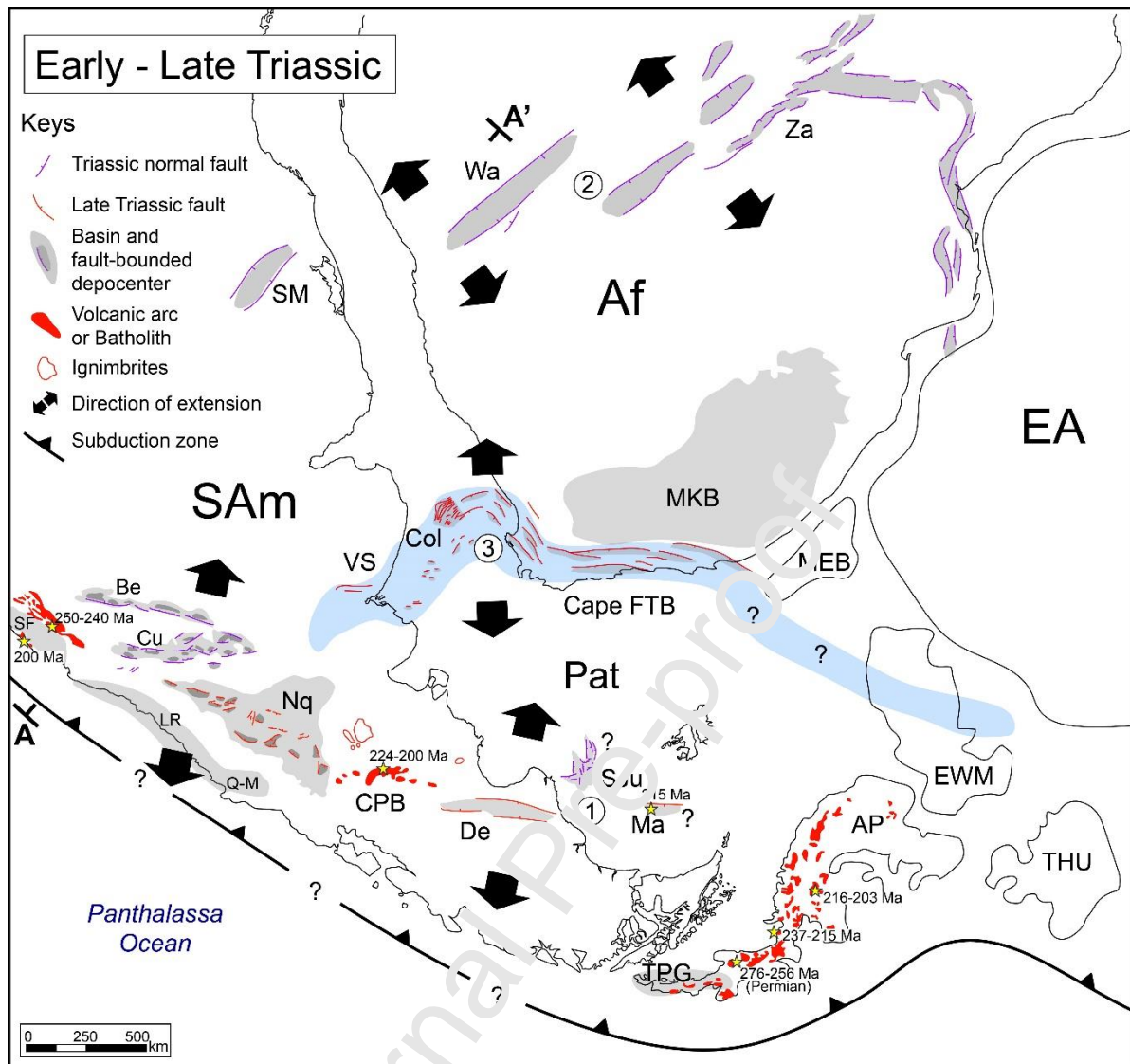
Fig. 8: Paleo-tectonic reconstruction of SW Gondwana at 200 Ma. Africa in its present-day position. Gondwana fit after: Daziel et al. (2013). Triassic volcanic arc in Central Chile after Oliveros et al. (2018), Central Patagonian Batholith (CPB, age after Rapela et al., 2005). Fore and intra-arc basins in Chile: SF: San Felix-Rivadavia basin, LR: La Ramada, Q-M: El Quereo-Los Molles basin (after Charrier et al., 2014). Volcanic arc in the Antarctic Peninsula (AP) and extension of the Trinity Peninsula Group (TPG) basin the after Bastias et al. (2020), Storey et al. (1992), Millar et al. (2002), Flowerdew et al. (2006), and Riley et al. (2012). Basins develop in a back-arc: Cuyo (Cu), Bermejo (Be), faults after Uliana et al. (1995); or intracratonic setting: Santa María (SM), Waterberg (Wa), Zambezi (Za), after Zerfass et al. (2004), San Julián (SJ, after Micucci et al., 2011). Late Triassic-Early Jurassic basins: Neuquén (NQ, Precuyano cycle, faults after Bechis et al., 2014), Deseado (De) and Malvinas (Ma) basins after Uliana et al. (1989). The previously compressive faults of the Ventania (VS) - Cape Permian-Early Triassic fold and thrust belt (FTB, in blue) have been extensionally reactivated in the Colorado (Col) and Cape area (Lovecchio et al., 2018; Paton, 2006). MKB: Main Karoo basin. Tectonic blocks: South America (Sam), Patagonia (Pat), Africa (Af), Maurice Ewing Bank (MEB), Eastern Antarctica (EA), Ellsworth-Whitmore Mountains (EWM), Antarctic Peninsula (AP), Thurston Island-Eights Coast (THU). 1, 2 and 3 are different groups of basins referred in the text.
