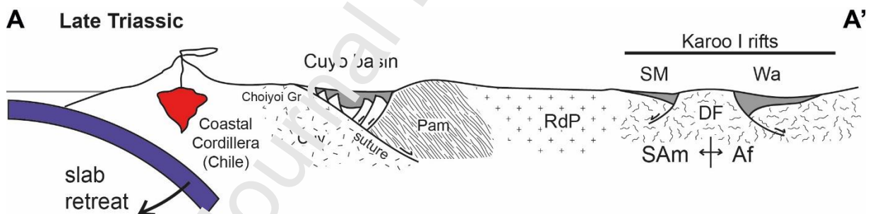
Fig. 9: Schematic cross-section of the SW Gondwana margin for the Late Triassic (not to scale). See location in Fig. 8. The magmatic arc is represented by the Coastal Cordillera Batholith (Chile); extension took advantage of the Early Paleozoic Cuyania suture to form the Cuyo basin; Intracontinental rifting in Africa produced the Karoo I rifts. After Ramos and Kay (1991), Oliveros et al. (2018) and Zerfass et al., (2004). See keys on cratones and tectonic blocks in Fig. 2.
