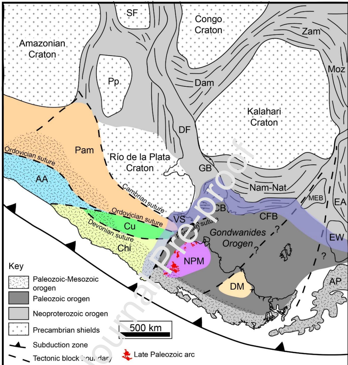
Fig. 2: Simplified structural scheme of SW Gondwana at the end of the Paleozoic, with a detail of cratons, terranes and metamorphic belts, after Gray et al. (2008); Ramos (2010); Pankhurst et al. (2006); P ngaro and Ramos (2012); and Lovecchio et al. (2018). Main Precambrian mobile belts: Dom Feliciano (DF), Gariep (GB), Namaqua-Natal (Nam-Nat), Mozambique (Moz). Main Paleozoic accreted terranes (in different colours): Pampia (Pam), Cuyania (Cu), Arequipa-Antofalla (AA), Chilenia (Chi). Other Tectonic blocks: Paran -Panema (Pp), Sao Francisco (SF), North Patagonian Massif (NPM), Deseado Massif (DM), Eastern Antarctica (EA), Antarctic Peninsula (AP). Permian-Triassic fold and thrust belt (purple): Ventania system (VS), Prerift of the Colorado basin (CB), Cape Fold Belt (CFB), Ellsworth-Whitmore Mountains (EW). UTM Projection. Undeformed plates, after Ramos (1999, 2008).
