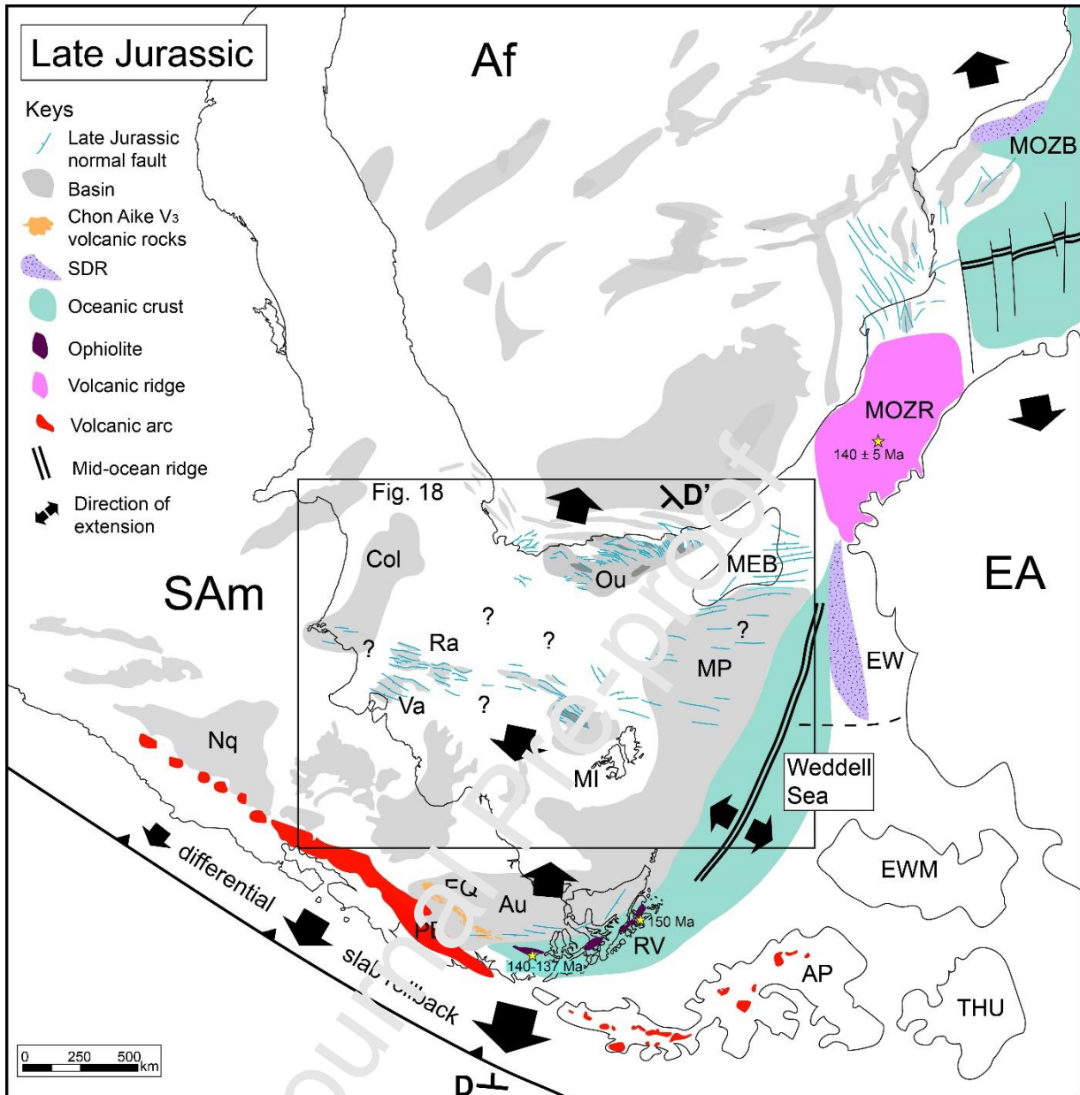
Fig. 12: Paleo-tectonic reconstruction of SW Gondwana in the Late Jurassic. Gondwana fit after König and Jokat (2006). The Mozambique channel opens as Antarctica moves south. Wrenching along the South America-Antarctica limit ends with seafloor spreading and the origin of the Weddell sea. Faults in the Mozambique area after Macgregor (2017) Mozambique Ridge (MOZR) age after Mueller and Jokat (2017). The Rocas Verdes (RV) back-arc basin develops to the west of the Austral basin. Schematic Patagonian Batholith (PB) after Rapela et al. (2005). Oceanic crust ages after Mukasa and Dalziel (1996) and Stern et al. (1992). Oblique rifting produced the formation of the Rawson/Valdés (Ra/Va) and Outeniqua (Ou) basins in the core of the Late Paleozoic Gondwanides orogen. Wrenching along the future Agulhas-Malvinas (Falkland) fracture zone (AMFZ) will release South America from Africa and produce the breakup along the Neoproterozoic mobile belt. The black rectangle shows the location of the zoom presented in Fig. 18.
