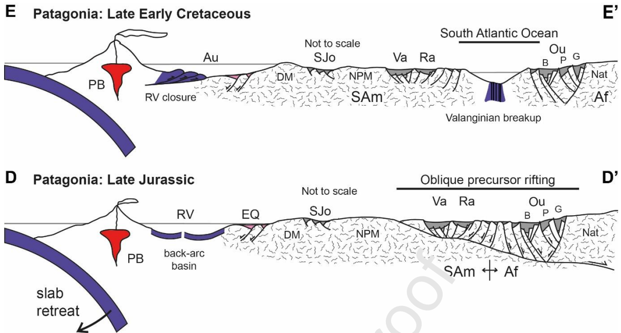
Fig. 13: Schematic cross sections of the SW Gondwana margin (not to scale). D-D' is a transect across SW Patagonia in the Late Jurassic, with a magmatic arc represented by the Patagonian Batholith, retroarc extension marked by the emplacement of El Quemado complex and equivalents and spreading in the Rocas Verdes back-arc basin. Oblique rifting in the Rawson/Valdés and Outeniqua basin was precursor of the South Atlantic opening. See location in Fig. 12. Modified after Ramos (1993), Continanzia et al. (2011) and Broad et al. (2012). E-E' is a generalized transect across SW Patagonia in the Early Cretaceous ( sensu lato ), compression in the SW Gondwana margin is evidenced by the closure of the Rocas Verdes basin and onset of a foreland setting in the Austral-Magallanes basin in the Late Early Cretaceous. Spreading in the southern South Atlantic Ocean initiated in the Valanginian. See partial location in Fig. 15. Keys for basins and tectonic blocks as in Fig. 2, 3, 5 and 15.
