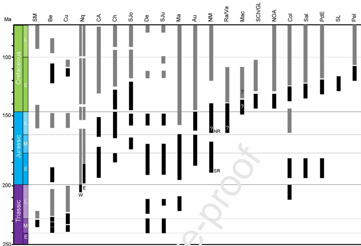
Fig. 4: Rifting chronology chart for the main Mesozoic basins of SE South America. Black bars represent active rifting, while grey bars represent sag or other tectonic scenarios (e.g. drift, foreland). Santa María (SM), Bermejo (Be), and Cuyo basin (Cu) after Kokogian and Mancilla (1989); Zeffass et al. (2004); Barredo et al. (2012) and Colombi et al. (2015). Neuquén basin (Nq) after D'Elia et al. (2015), references therein and authors' interpretation. Cañadón Asfalto (CA) after Cúneo et al. (2013) and Figari et al. (2015). Chubut Liassic basin after Suárez and Márquez (2007) and references therein, San Jorge Gulf basin (SJo) after Fitzgerald et al. (1990), and Lanzetta et al. (2004). Deseado (De) and San Julián (SJu) basins after Figueiredo et al. (1996). Austral/Magallanes (Au) includes the Late Jurassic Rocas Verdes basin, age after Pankhurst et al. (2000) and Calderón et al. (2013). Malvinas (Ma) after Galeazzi (1998) and Lovecchio et al. (2019); North Malvinas (North Falkland) basin after Ramos et al. (2017); and Lohr and Underhill (2015). Rawson/Valdés basin (Ra/Va) after Continanzia et al. (2011). Macachín basin (Mac) is undrilled, thus rifting age is poorly constrained. Sierras Chicas and General Levalle basins in Córdoba (SCh/GL) after Lagorio et al. (2016); Schmidt et al. (1995); and Webster et al. (2004). Northwestern Argentina Cretaceous basin (NOA) after Starck (2011) and references therein, age after Galliski and Viramonte (1988). Colorado (Col), Salado (Sal), and Punta del Este (PdE) basins after Lovecchio et al. (2018); Gerster et al. (2011); and Loegering et al. (2013). Santa Lucía basin (SL) after Veroslavsky, (1999). Pelotas (Pel) after Stica et al. (2014) and references therein.
