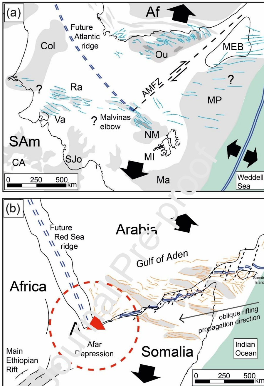
Fig. 18: Comparison of a) Late Jurassic oblique rifting in the southern South Atlantic area; and b) Cenozoic oblique rifting in the Gulf of Aden (after Leroy et al., 2012 and Mohriak and Leroy, 2013).
