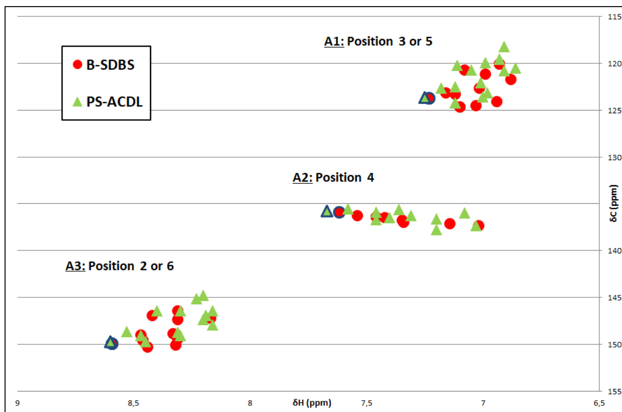
Figure 1. \{^1H, ^{13}C\} HSQC spectra of pyridine derivatives simulated by PS-ACDL and given by B-SDBS.
