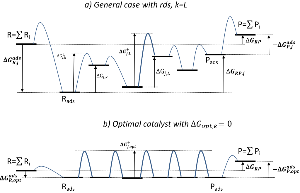
Scheme 1 : Energy profiles a) for the general case of a non-optimal catalyst with rate determining step k=L , and b) for the optimal catalyst for which |\Delta G_{k,opt}| = |\Delta G_{L,opt}| = 0 for 1 \leq k \leq N
