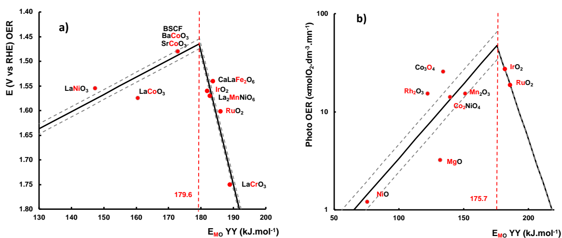
Figure 1 Volcano plots for the electrocatalytic oxygen evolution reaction (OER) (a) and the photocatalytic OER (b). Experimental activity patterns in ordinates from 16,17 in OER, and 18,19 in photocatalytic OER. In abscissae, DFT calculated E_{MO} descriptors computed according to the Yin Yang method 3 with target atoms indicated in red when necessary. The regression lines, connecting data points, materialize the left- and right- hand sides of the
