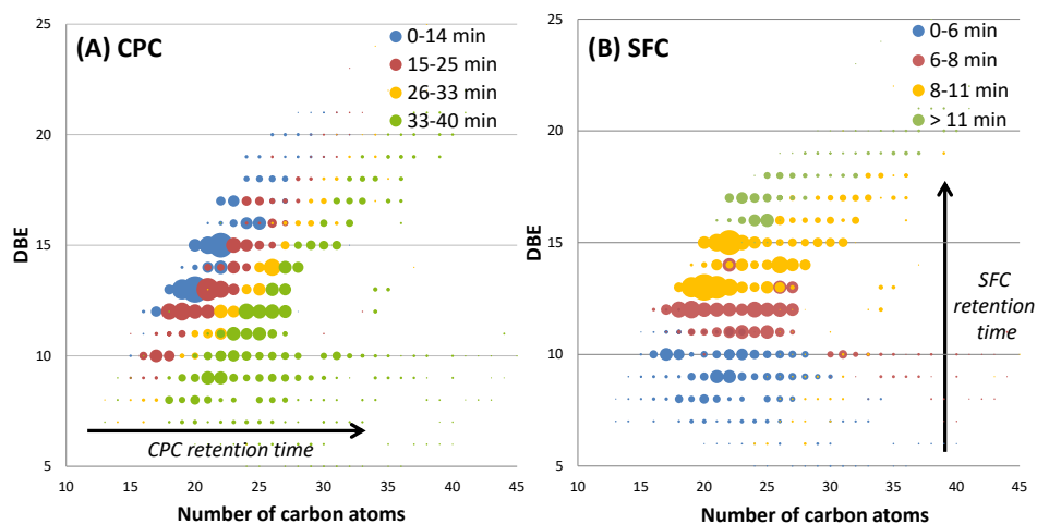
Figure 6: DBE as a function of the number of carbon atoms for C_xH_y compounds detected in VGO 1. Colour scales represent the retention times of (A) CPC, (B) SFC and size of the points is related to the intensity of the compounds on MS spectra.
