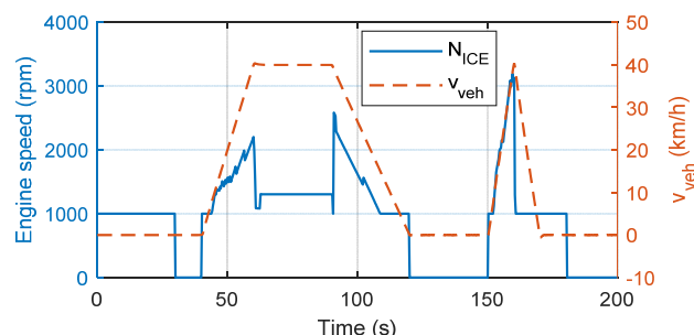
Figure 14: illustration of the Stop and Start system operation (conventional mode)
