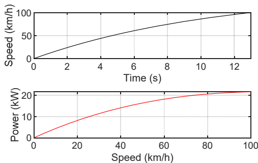
Figure 5: Power request for 0-100 kph acceleration criteria
