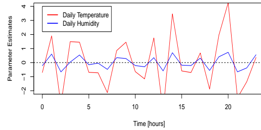
(b) Adaptive fused group LS solution
