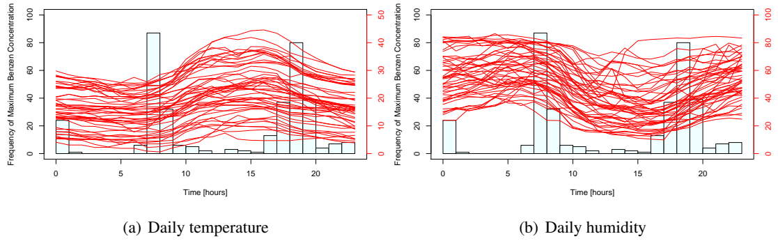
Figure 2. Daily temperature profiles (left panel) and daily humidity profiles (right panel) for 50 randomly selected days out of 357 available days with full profiles in total. In addition, the maximum benzene concentration is recorded for each day and the corresponding time of the maximum occurrence (in hours) is given in terms of the frequency histograms in both panels.
