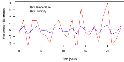
(a) Fused group LS solution
