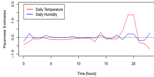
(c) Fused group quantile solution
