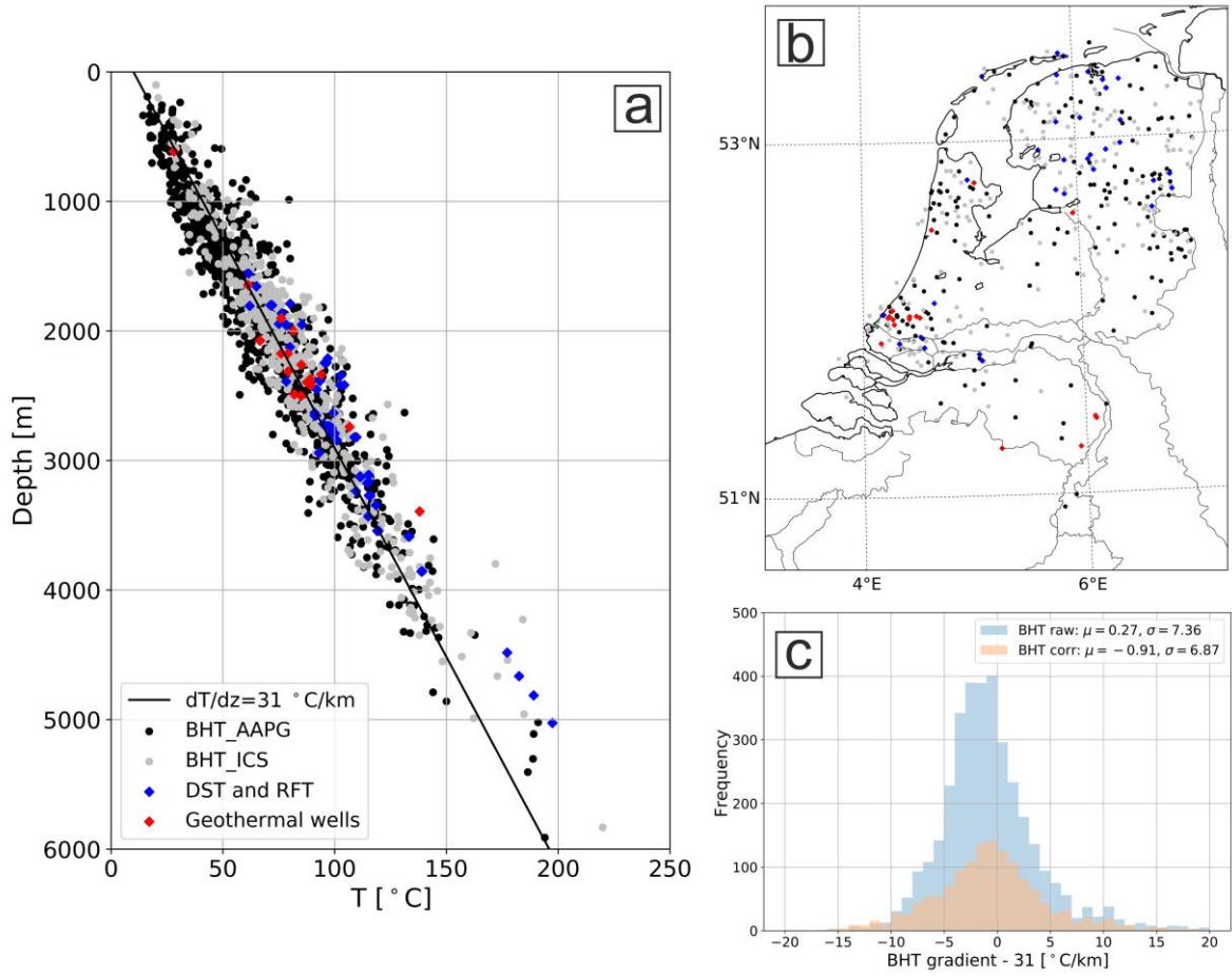
201 202 Figure 3. Temperature dataset including BHTs, DSTs, RFTs and production temperatures from geothermal wells 203 modified after Bonté et al. (2012) (a). BHT_ICS: BHTs corrected with analytical method, BHT_AAPG: BHTs 204 corrected with statistical method. The temperature measurements were collected from wells drilled in the 205 onshore Netherlands (b). In case of multiple measurement types in a single well, the one with the lower 206 uncertainty is shown in (b). The misfit of raw and corrected BHT gradients with the average Dutch geotherm are 207 shown in (c), with the mean and standard deviation of the fitted Gaussian functions.
