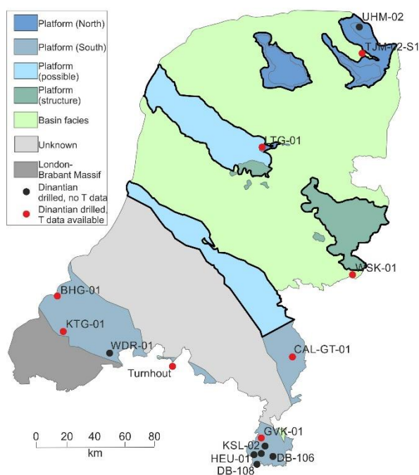
333 334 Figure 6. Map showing the locations of the Dinantian carbonate platforms and other rocks of Dinantian age 335 modified after Kalkman (2016). We use scaling of the thermal conductivity to approximate the thermal effects of 336 convection. Outlined in black are the areas below the carbonate platforms for which we scaled the thermal 337 conductivity values.
