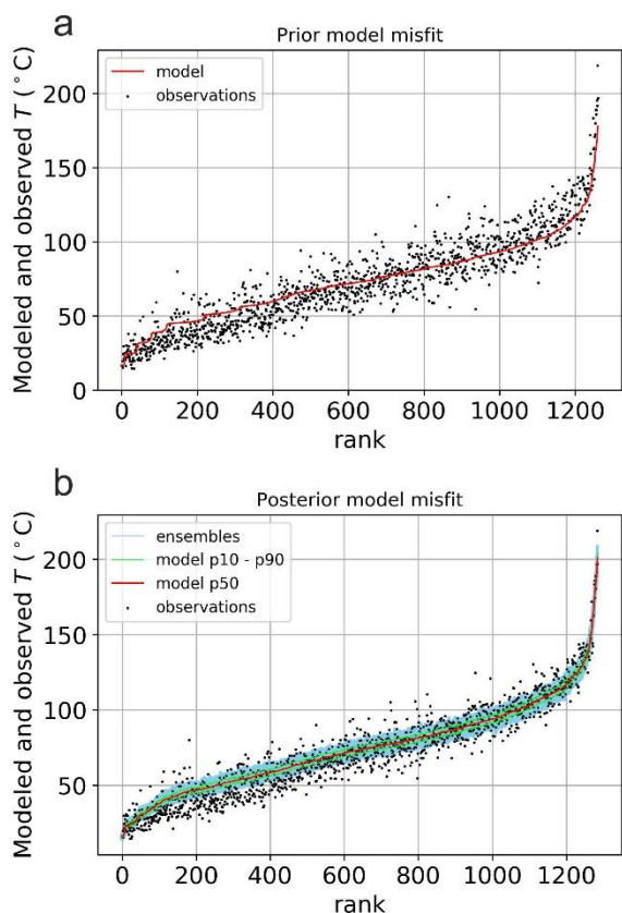
540 541 Figure 11. Distribution of the modeled and observed temperatures ranked by the modeled temperatures at the 542 observation points for the prior (a) and posterior (b) models. Temperature measurements are marked by black 543 dots. The red curves indicate the model results (in (b) the P50 values), the green lines in (b) are the P10 and P90 544 values. The blue interval in (b) indicates the modeled temperatures for all the 600 ensemble members of the last 545 iteration.
