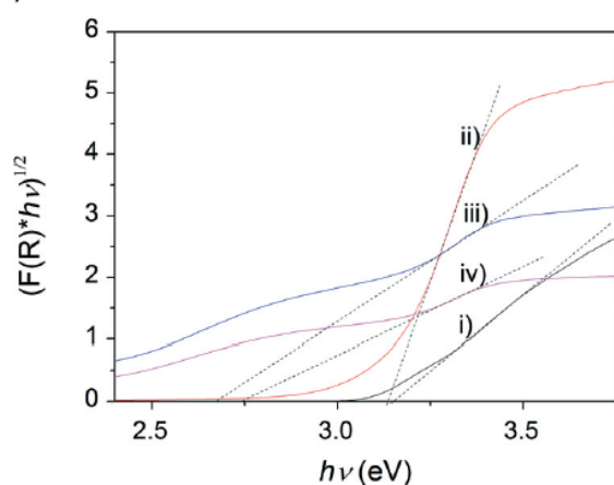
Fig. 1 a) TEM micrographs, b) Tauc plots and c) adsorption spectra of the investigated samples: i) P25 \text{TiO}_2 , ii) undoped \text{TiO}_2 , iii) \text{N-TiO}_2(\text{G}) and iv) \text{N-TiO}_2(\text{P}) .
