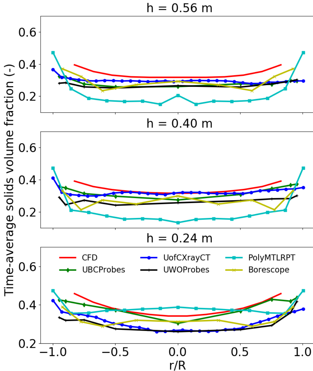
Fig. 12. Comparison of radial solids volume fraction at three heights obtained by tracer particle experimental measurements and CFD bulk simulations for U_g=0.40 \text{ m/s} .
