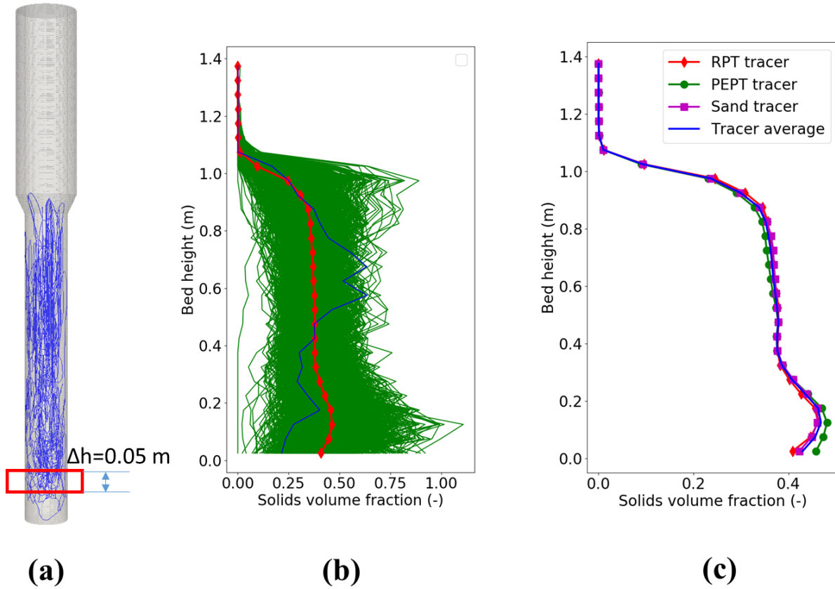
Fig. 7(a) Trajectory of 1 of 1000 simulated RPT tracer particles for a superficial gas velocity of 0.4 m/s; (b) Cross-section averaged solids volume fraction from one RPT tracer particle (blue line), the other 999 RPT tracer particles (green line) and the average solids volume fraction of the 1000 RPT tracer particles (red line); (c) Average solids volume fraction profiles of three different types of tracer particle and corresponding average profiles.
