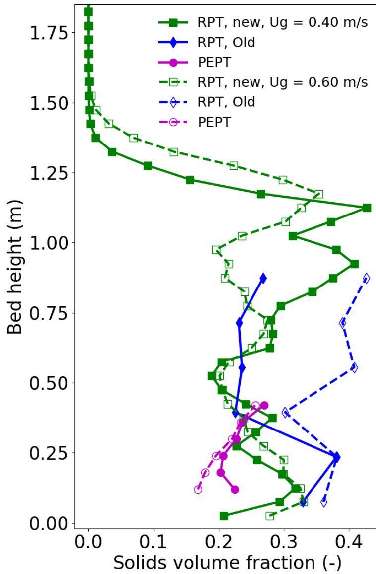
Fig. 13 Vertical profile of cross-sectional average solids volume fraction along bed predicted by RPT and PEPT method calibrated based on this research.
