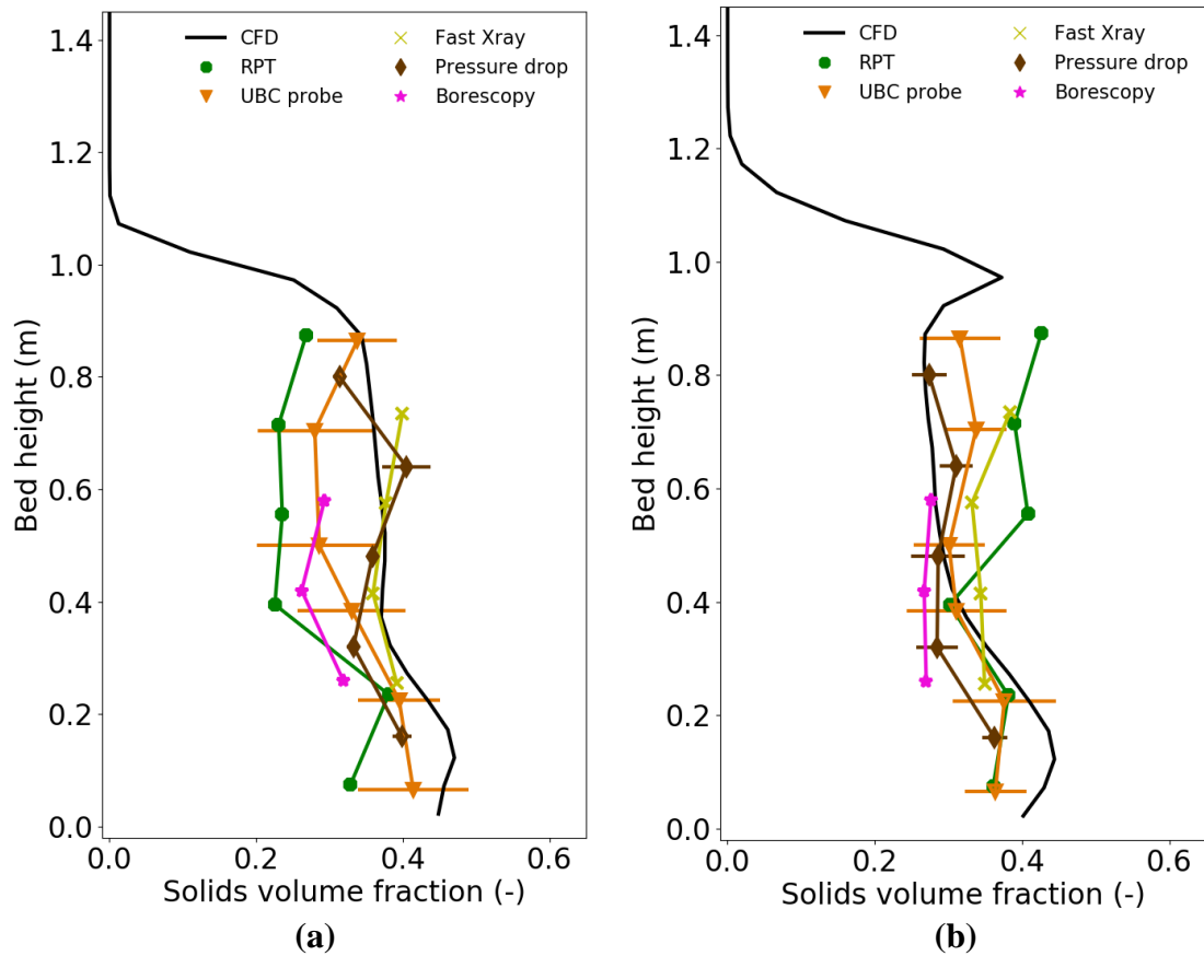
Fig. 9. Comparison of cross-sectional average solids volume fraction along bed provided by simulation and different experimental techniques: (a) U_g=0.40 m/s; (b) U_g=0.60 m/s.
