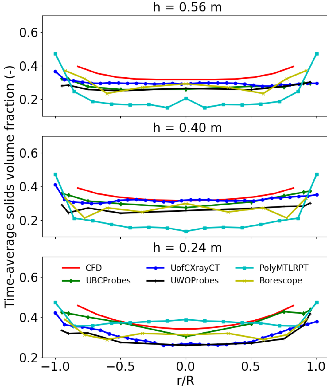
Fig. 12. Comparison of radial solids volume fraction at three heights obtained by tracer particle experimental measurements and CFD bulk simulations for U_g=0.40 m/s.
