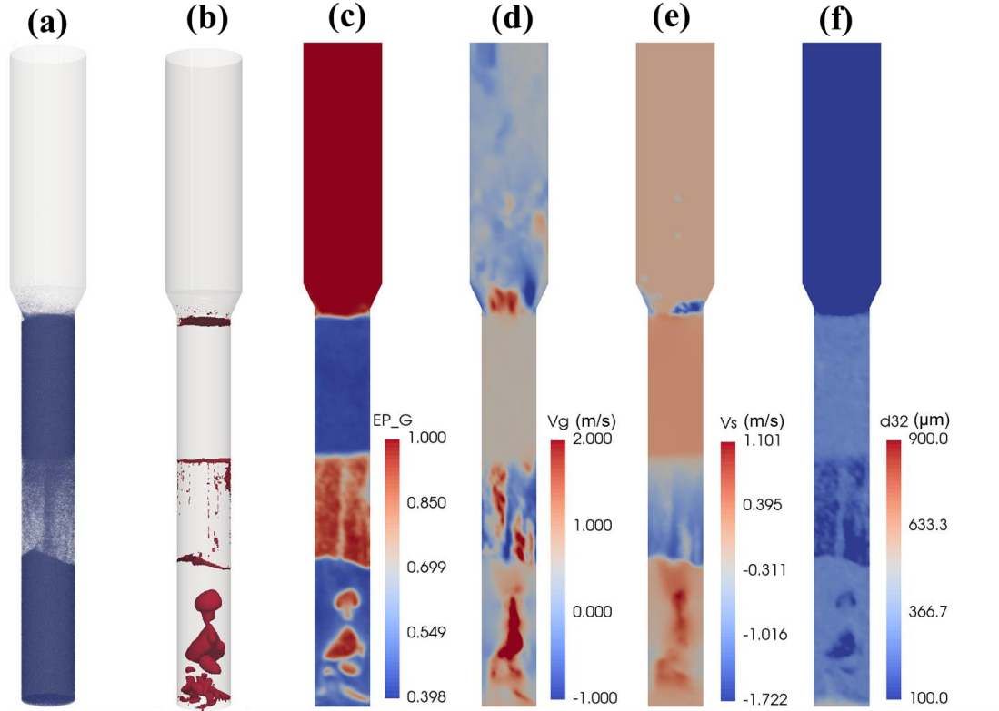
Fig. 5 Transient simulation results at t=82.70 s: (a) Particle distribution along the bed; (b) contour plot of voidage of 0.65; (c) local voidage; (d) vertical component of gas velocity (m/s); (e) vertical component of solid velocity (m/s); and (f) mean particle diameter ( \mu\text{m} ) ( V_s : solid-phase vertical component of velocity calculated by averaging particle velocities in each fluid cell; d_{32} : Sauter mean diameter of particles in each fluid cell. ( U_g=0.40 m/s).
