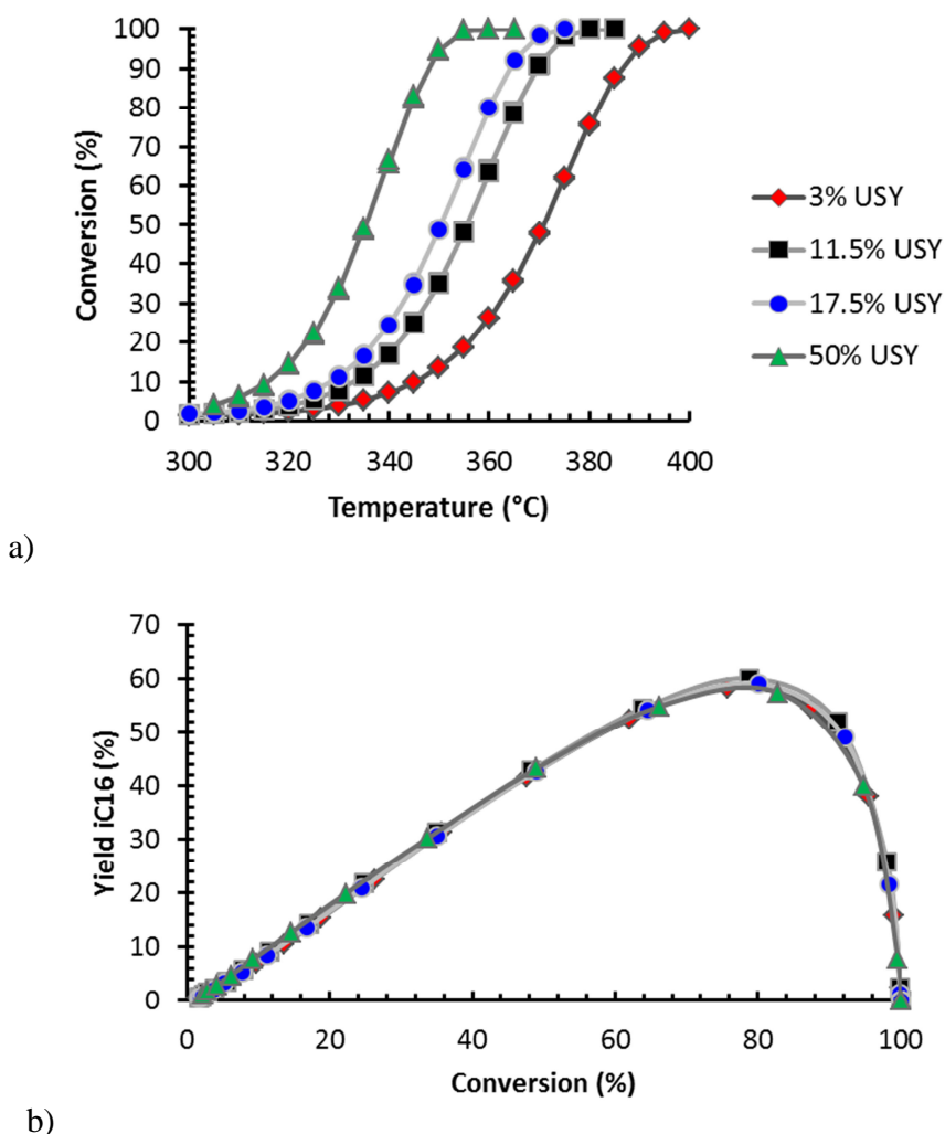
Figure 2. a) Conversion of n-C 16 in the presence of 750 ppm NH 3 over 1 wt% Pt-USY-Al 2 O 3 catalysts with different USY loadings. b) Yield of i-C 16 isomers as a function of conversion.
