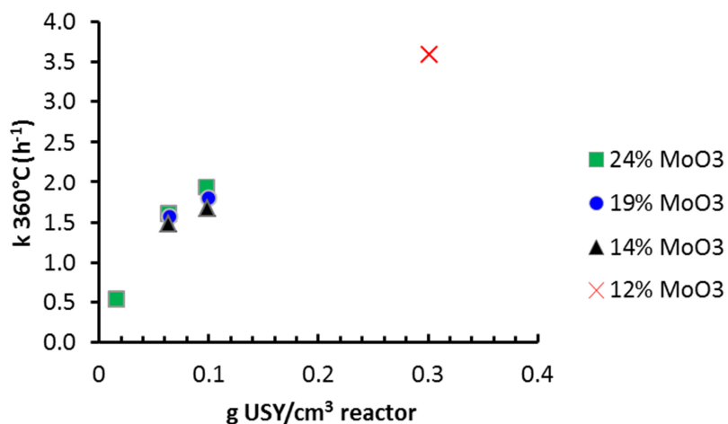
Figure 3. First order rate constant of hydroconversion of n\text{-C}_{16} over NiMo-USY- \text{Al}_2\text{O}_3 catalysts in the presence of 750 ppm \text{NH}_3 as a function of the USY content in the reactor.
