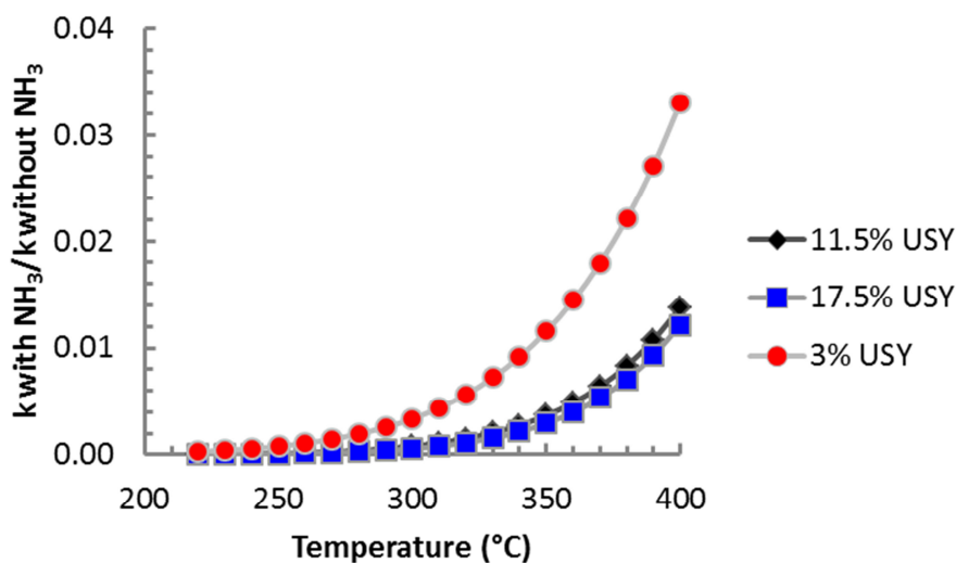
Figure 9. Ratio of rate constants of balanced Pt-USY-Al 2 O 3 catalysts (extrapolated from an Arrhenius equation) in the presence and absence of NH 3 .
