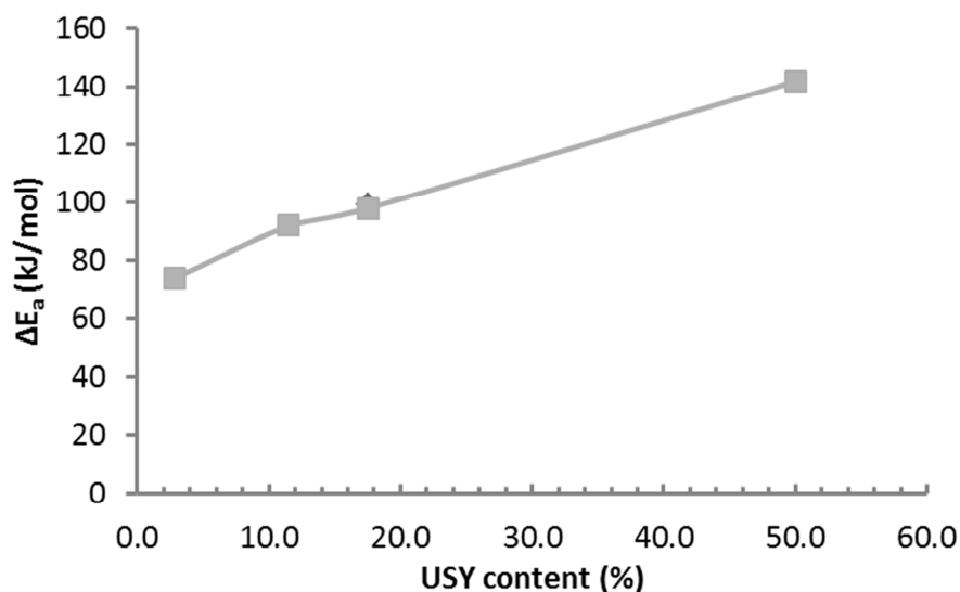
Figure 8. Difference in the activation energy of Pt-USY-Al 2 O 3 catalysts in the presence and absence of NH 3
