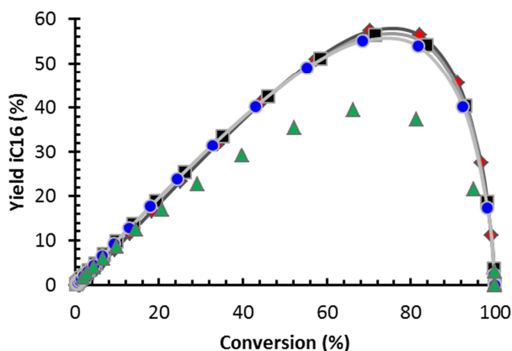
Figure 1. a) Conversion of n\text{-C}_{16} over 1 wt% Pt-USY- \text{Al}_2\text{O}_3 catalysts with different USY loadings. b) Yield of i\text{-C}_{16} isomers as a function of conversion.
