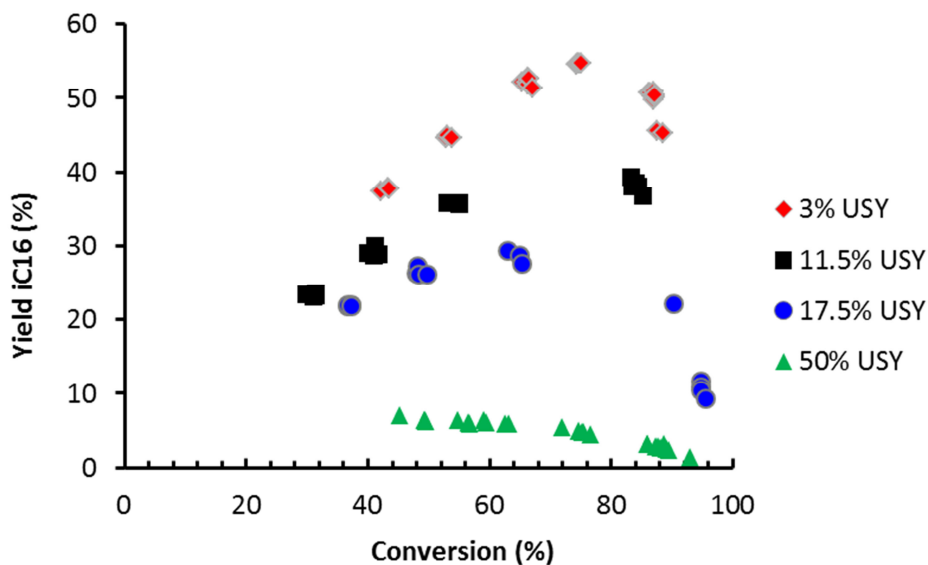
Figure 4. i\text{-C}_{16} yield as a function of conversion at 360^{\circ}\text{C} over NiMo-USY- \text{Al}_2\text{O}_3 catalysts in the presence of 750 ppm \text{NH}_3 . For each zeolite loading, the catalyst with the highest available \text{MoO}_3 content was represented.
