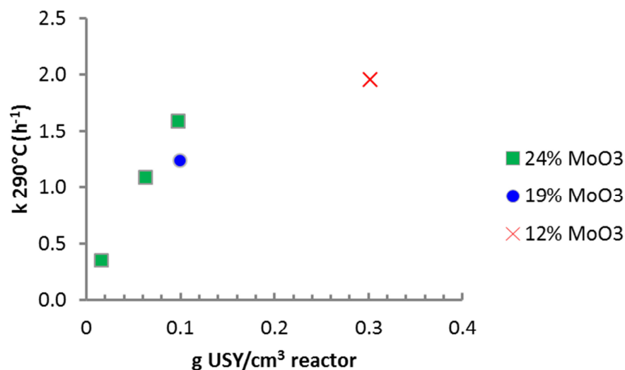
Figure 6. First order rate constant of hydroconversion of n-C 16 over NiMo-Al 2 O 3 -USY catalysts at 290°C as a function of the USY content in the reactor.
