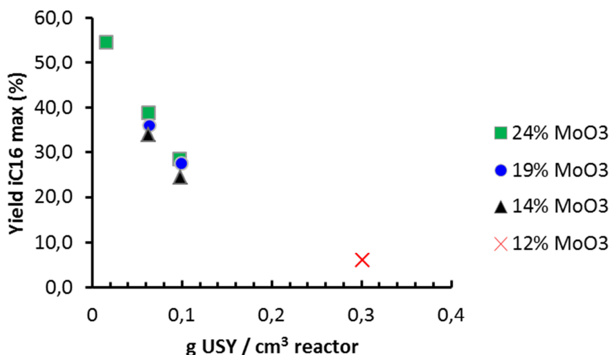
Figure 5. Maximum isomer yield versus zeolite content: NiMo-USY-Al 2 O 3 catalysts in the presence of 750 ppm NH 3
