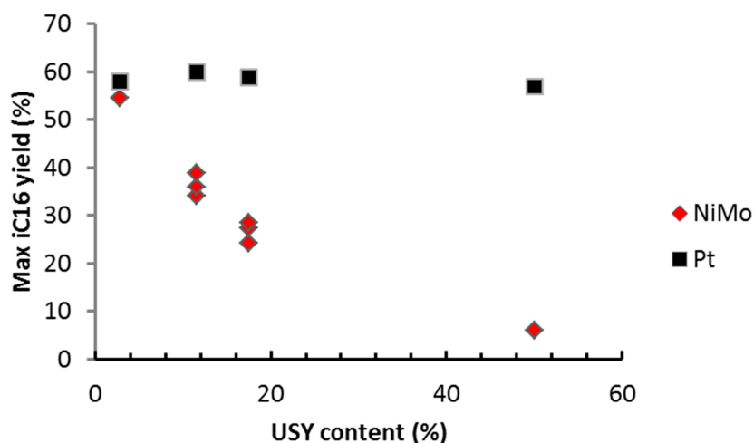
Figure 10. a) Rate constant of Pt- and NiMo-USY-Al 2 O 3 catalysts at 360°C, in the presence of NH 3 ; b) maximum i-C 16 yield as a function of USY content, in the presence of NH 3 .
