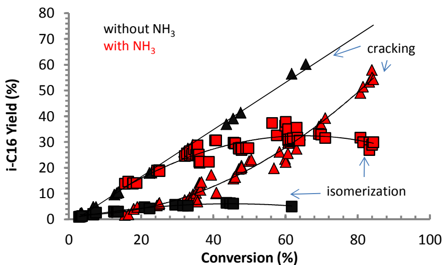
Figure 7. Yield of cracking products (triangles) and i-C 16 (squares) as a function of conversion. Black symbols: reaction in absence of NH 3 , red symbols: reaction in presence of NH 3 . Catalyst NiMo-USY-Al 2 O 3 (17.5 wt% USY, 19 wt% MoO 3 )
