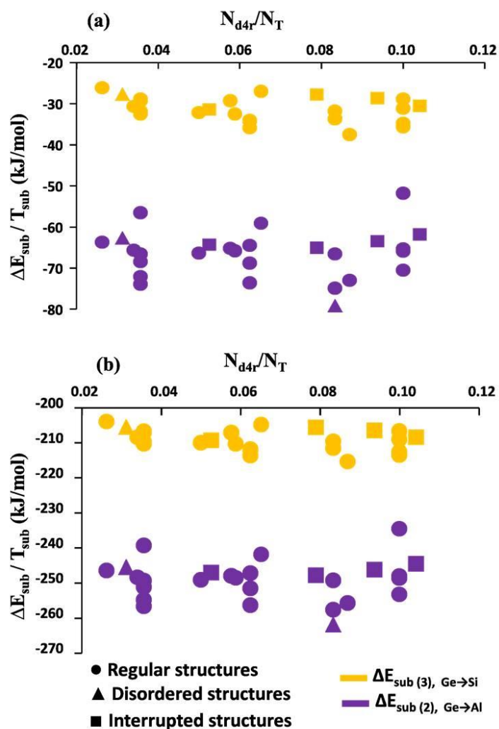
Figure 7: Energies of full substitution of Ge for Si ( \Delta E_{\text{sub}}(3), \text{Ge} \rightarrow \text{Si} ) departing from Ge occupying the full d4r (yellow) and of Ge for Al ( \Delta E_{\text{sub}}(2), \text{Ge} \rightarrow \text{Al} ) departing from Ge occupying half of the d4r with alternation (purple), normalized to the number of substituted T sites, using (a) hydroxides and (b) chlorides against the number of d4r in the structures over the total T sites ( N_{d4r}/N_T ). Spheres, triangles and squares correspond to regular, partially disordered and interrupted zeolite structures, respectively.
