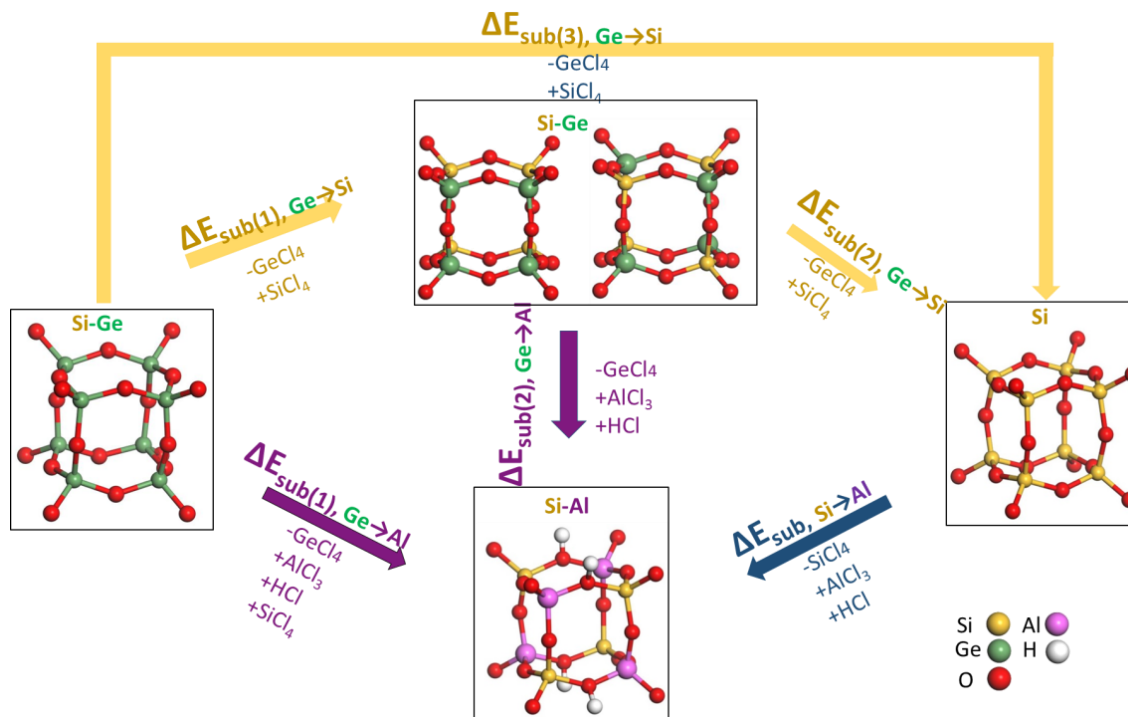
Figure 6: Substitution scheme of Ge for Si and Al using chlorides. The d4r part of the structures only are shown, the other parts of the structure (with T sites occupied by Si only) are omitted for the sake of clarity and for generalization purposes.
