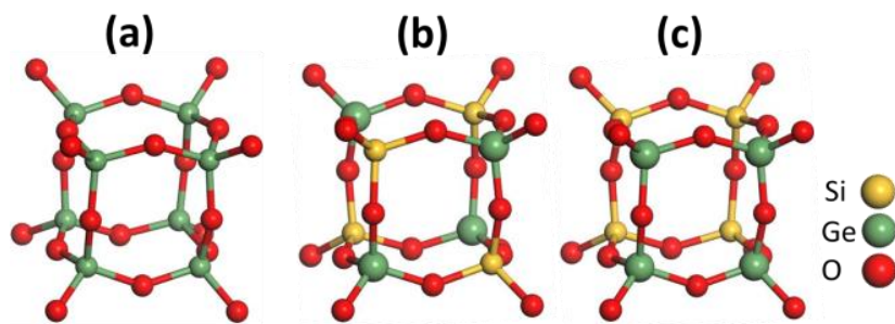
Figure 1: Ge and Si siting in d4r units: (a) Ge occupying all d4r, (b) Ge occupying half of the d4r with alternation with Si and (c) Ge occupying half of the d4r in a same s4r. The d4r part of the structures only are shown, the other parts of the structure (with T sites occupied by Si only) are omitted for the sake of clarity and for generalization purposes.
