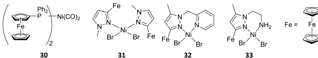
Figure 18. Iron containing nickel complexes
