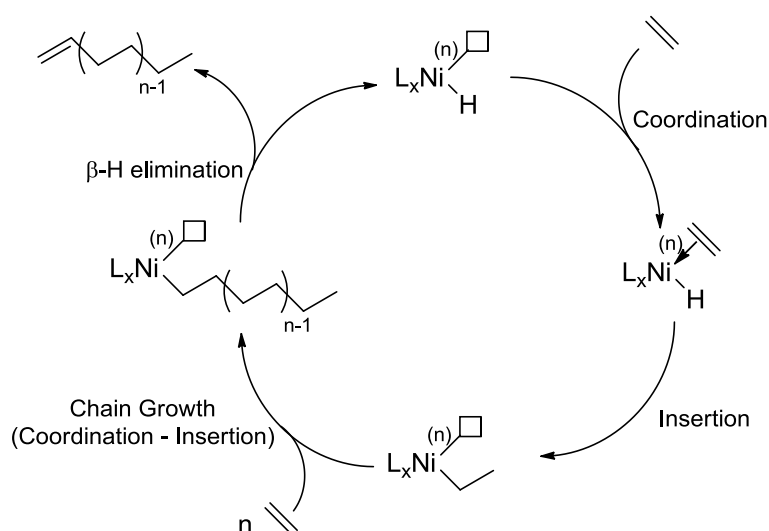
Scheme 8. Cossee-Arlman mechanism.
