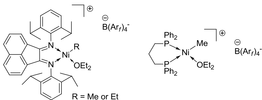
Figure 48. Examples of isolated cationic alkylnickel complexes
