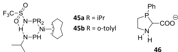
Figure 22. (P,O)-bidentate monoanionic based ligands and nickel complexes
