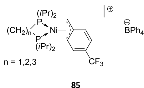
Figure 46. Examples of isolated cationic allylnickel complexes
