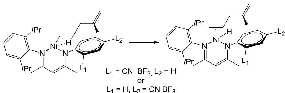
Scheme 19. Rojas et al. study on termination pathway in Cossee-Arlman mechanism
