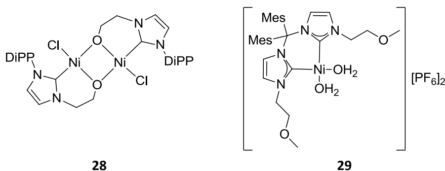
Figure 17. N-Heterocyclic carbene-based nickel(II) complexes
