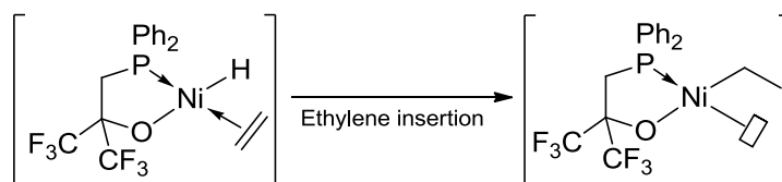
Scheme 11. ^1\text{H} NMR study of the reactivity of nickel hydride with ethylene
