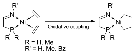
Scheme 20. Imino-phosphorane Ni complexes and their role in metallacycle formation
