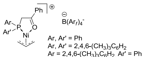
Figure 47. Examples of isolated cationic allylnickel complexes
