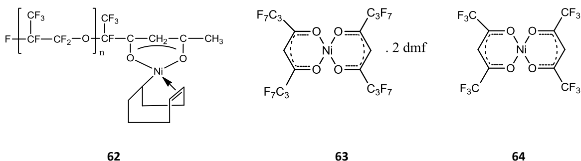
Figure 30. Perfluorinated Ni-complexes for FBS olefins oligomerization
