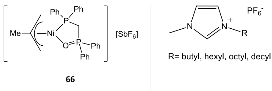
Figure 33. Weakly-coordinating ILs for the biphasic ethylene oligomerization using cationic Ni-complexes
