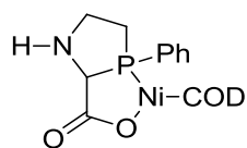
Figure 24. Suggested in situ -formed catalytic species for 46
