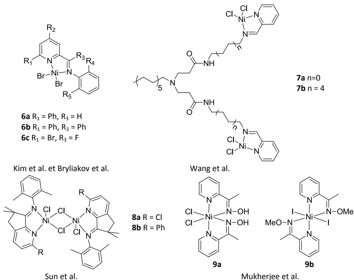
Figure 8. Iminopyridine and oxime nickel(II) complexes
