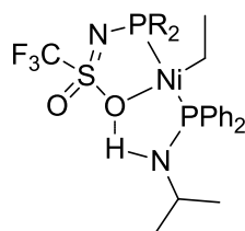
Figure 23. Suggested in situ -formed catalytic species for 45 (a. R = o-tol, b = iPr)
