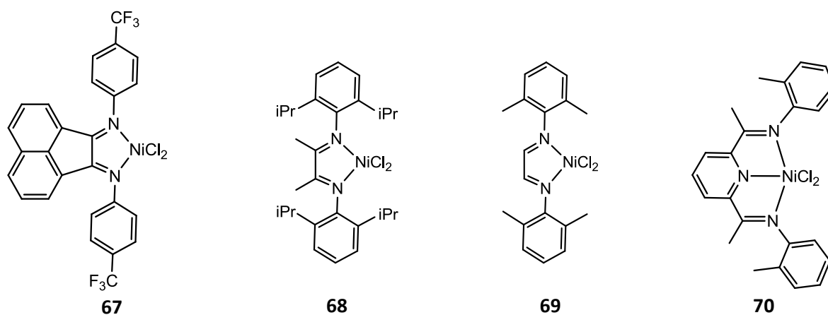
Figure 34. \alpha -diimine and bis-iminopyridine Ni(II) precursors
