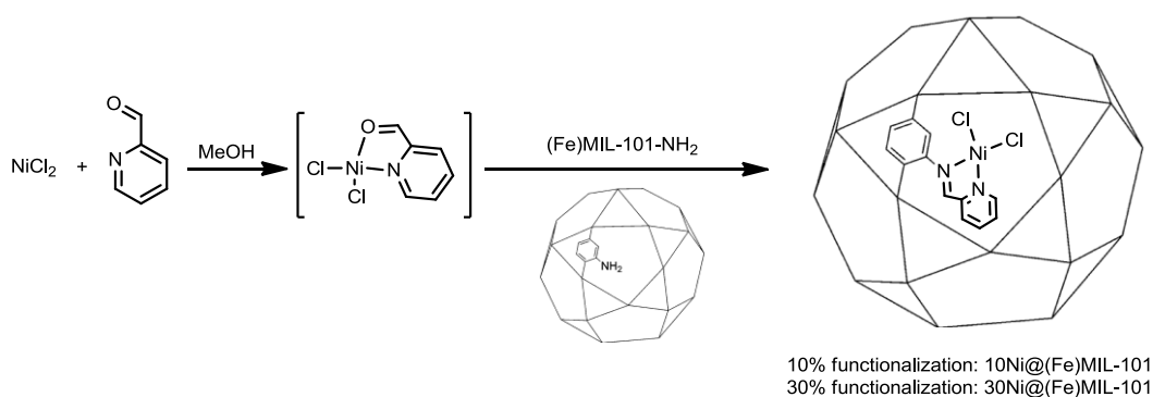
Scheme 2. Strategy for MixMOFs-Ni synthesis
