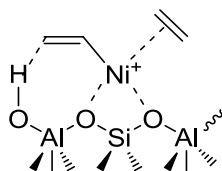
Figure 52. DFT-computed intermediate proposed in nickel active site generation in a SSZ-24 zeolite framework 26
