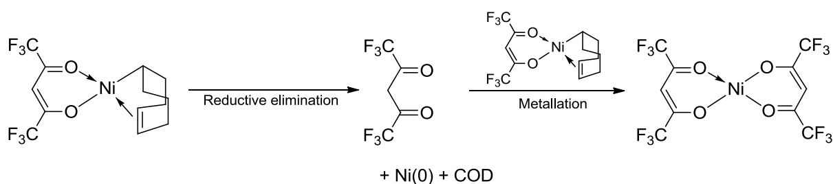
Scheme 21. Possible deactivation pathway for fluorinated-acetylacetonate Ni octadienyl catalysts
