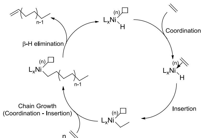
Scheme 8. Cossee-Arleman mechanism.
