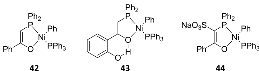
Figure 21. Reviewed (P,O)-bidentate monoanionic nickel complexes
