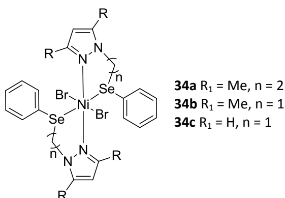
Figure 19. Selenium-functionalized pyrazole complexes
