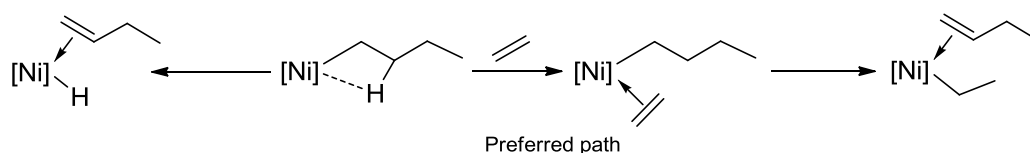
Scheme 17. Modeled insertion reaction of 1-butene on cationic [\text{Ni}(\text{L})_2(\text{butyl})]^+
