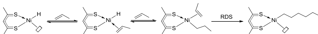
Scheme 16. Kinetic study of propylene dimerization with pentane-2,4-dithionato-based catalysts
