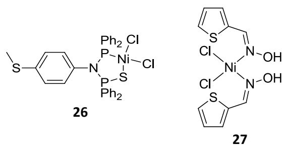
Figure 16. (P,S)- and (N,S)-based nickel(II) complexes
