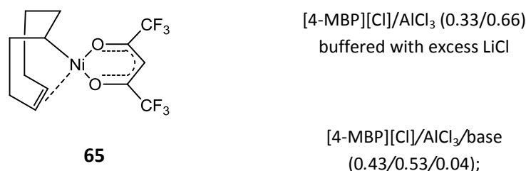
Figure 32. Buffered chloroaluminates
