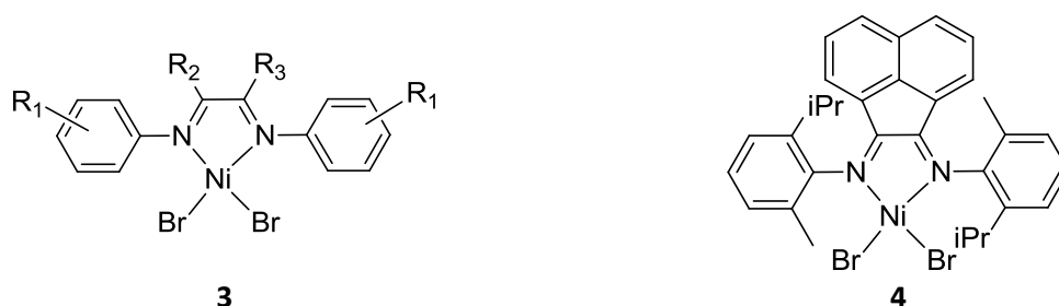
Figure 6. Brookhart type \alpha -diimine nickel(II) complexes
