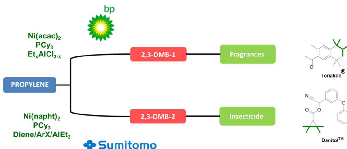
Figure 3. Selective dimerization of propylene to 2,3-DMB-1 and 2,3-DMB-2
