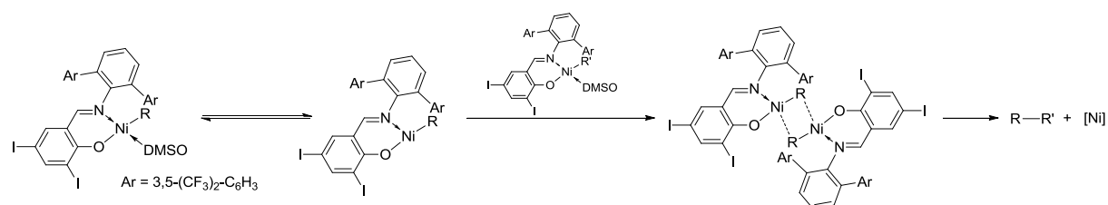
Scheme 22. Deactivation pathway involving heterocoupling
