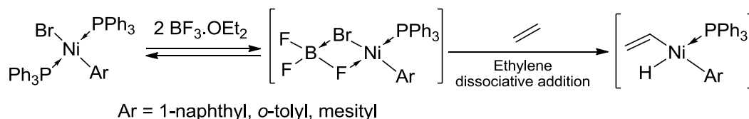
Scheme 12. Catalytic system formed by [\text{Ni}(\text{PPh}_3)_2(\sigma\text{-aryl})\text{Br}] and \text{BF}_3
