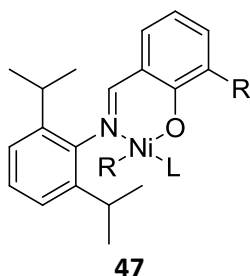
Figure 25. Reviewed (N,O)-phenoxyimine based nickel complexes
