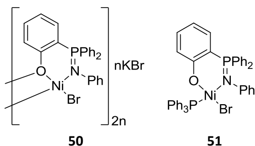
Figure 27. Iminophosphorane (N,O)-bidentate nickel(II) complexes
