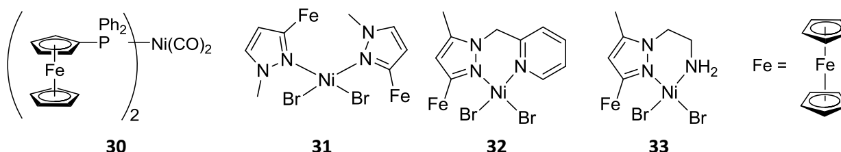
Figure 18. Iron containing nickel complexes
