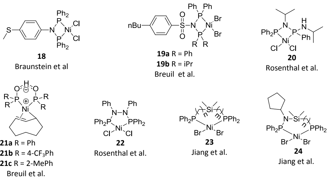
Figure 14. Diphosphine based nickel(II) complexes
