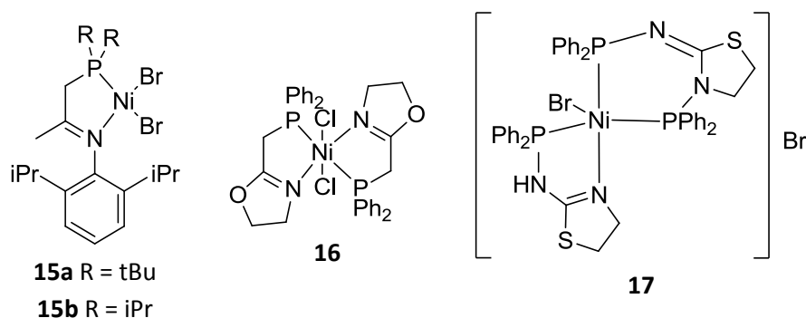
Figure 12. (P,N)-based nickel(II) complexes
