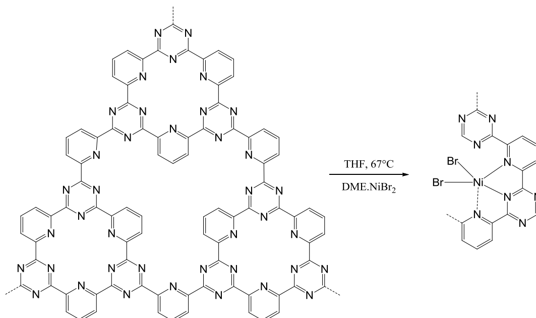
Scheme 5. Examples of synthesis of COFs and expected coordination of Ni 2+ to the nitrogen species in the frameworks
