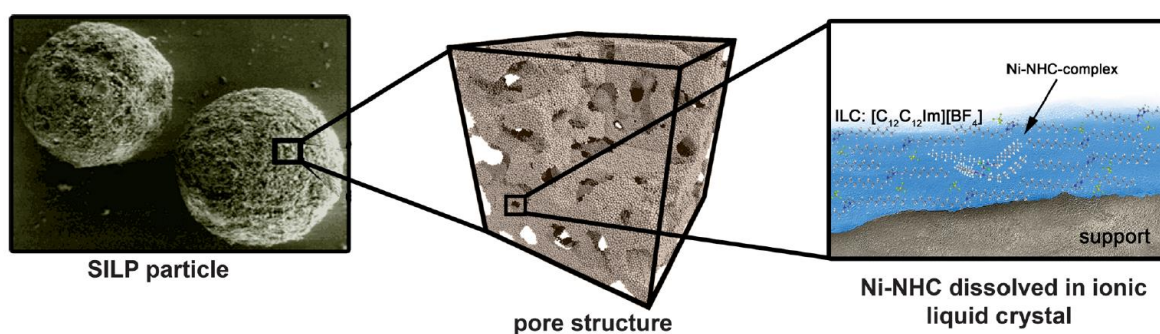
Figure 38. Schematic representation of a SILP material composed of ionic liquid crystal [C_{12}C_{12}Im][BF_4] with a Ni–NHC complex dissolved therein (reproduced with permission from ref 184. Copyright 2012 The Royal Society of Chemistry).
