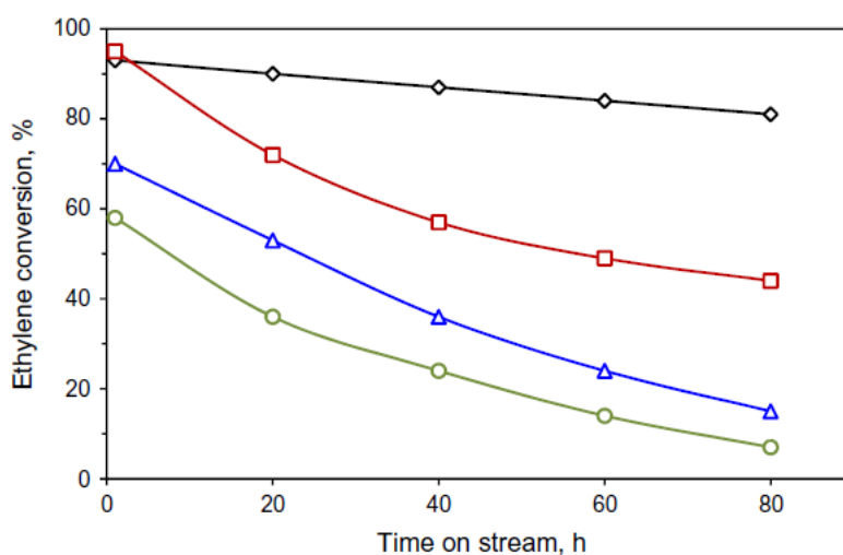
Figure 44. Activity profile of (◇) Ni-AlSBA-15 outperforming (□) Ni-MCM-41, (Δ) Ni-SiO 2 -Al 2 O 3 and (○) Ni-Y. (Reproduced with permission from ref 334. Copyright 2015 Elsevier)
