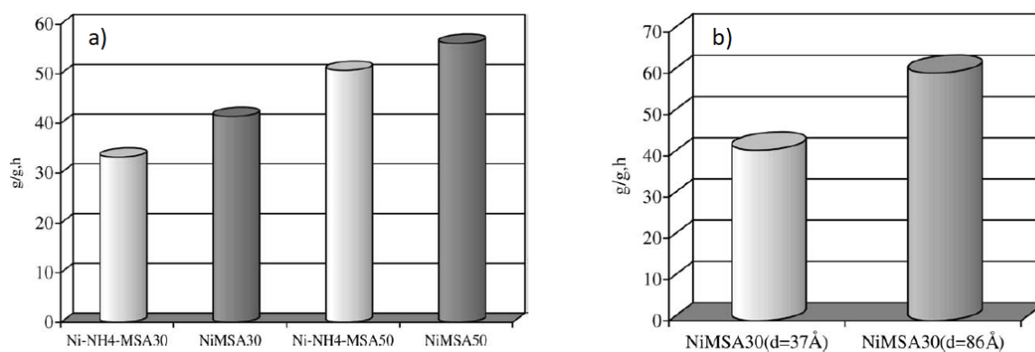
Figure 43. Effect of a) acidic properties and b) pore size on the catalytic activity of ethylene oligomerization at 150°C, 3.5 MPa after 60 minutes reaction time (Reproduced with permission from ref 325. Copyright 2004 Elsevier)
