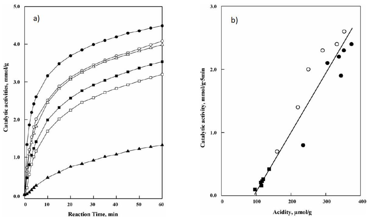
Figure 39. a) Catalytic activities of (■) 15-NiSO 4 /82-SiO 2 -Al 2 O 3 ; (●) 15-NiSO 4 /66-SiO 2 -Al 2 O 3 ; (▲) 20-NiSO 4 /SiO 2 against reaction time and b) Correlation between catalytic activity for ethylene
