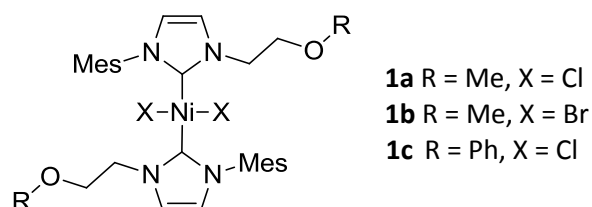
Figure 4. Ether functionalized NHC complexes
