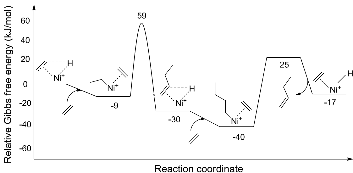
Figure 45. Mechanistic proposition for Ni/SSZ-24 catalyzed ethylene oligomerization based on DFT
