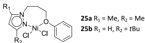
Figure 15. Neutral (N,O)-based nickel(II) complexes
