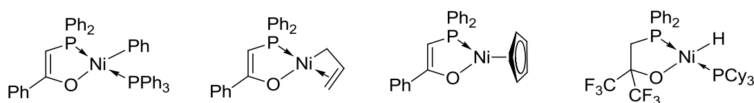
Figure 49. Examples of single site organometallic active nickel complexes
