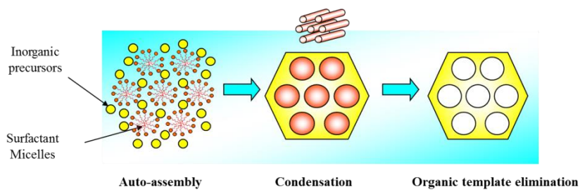
Scheme 6. Synthesis scheme for MCM-41 mesoporous materials
