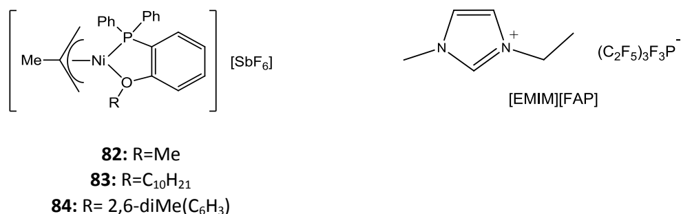
Figure 37. Composition of the SILP catalyst system used for ethylene dimerization
