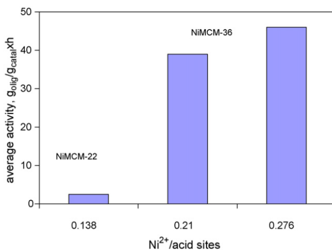
Figure 42. Effect of the \text{Ni}^{2+} /acid sites ratio on the catalytic activity of NiMCM-22 and -36 after 30 minutes (150°C, 40 bar) (Reproduced with permission from ref 311. Copyright 2008 Elsevier)
