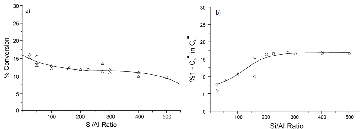
Figure 40. a) Ethene conversion and b) 1-Hexene selectivity as a function of Si/Al ratio of the support. T = 100 °C, P = 1.5 MPa, MHSV = 4 h -1 , and time-on-stream = 280 min. (Reproduced with permission from ref 281. Copyright 2003 Elsevier)
