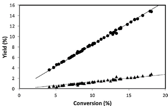
Figure 41. Experimental observations (symbols) and model simulations (lines) for butene yield (● and full line) and hexene yield (▲ and dashed line) as function of ethylene conversion (443-503 K, 0.15-0.35 MPa) (Reproduced with permission from ref 286. Copyright 2015 Elsevier)
