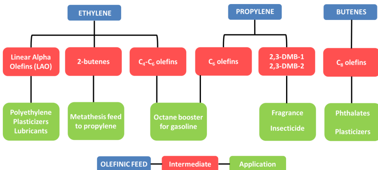
Figure 1. Oligomerization of light olefins to fuels and petrochemical intermediates and their applications
