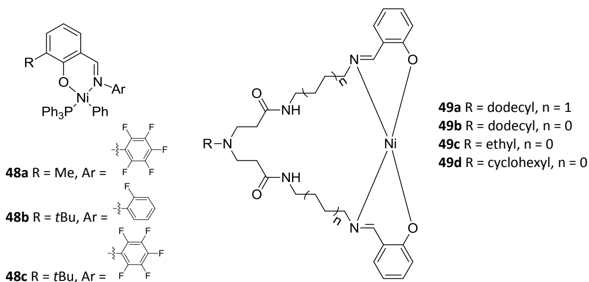
Figure 26. Salicylaldimine-based nickel(II) complexes
