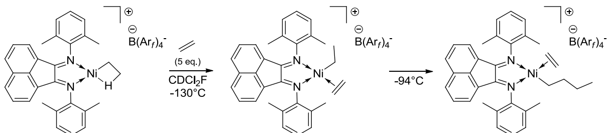
Scheme 14. Brookhart type complex reactivity with ethylene
