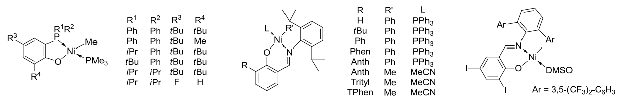
Figure 50. Examples of neutral active nickel complexes bearing bidentate monoanionic ligands
