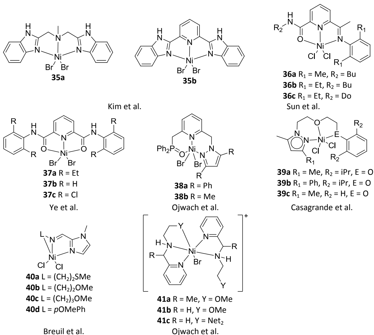
Figure 20. Tridentate nickel complexes
