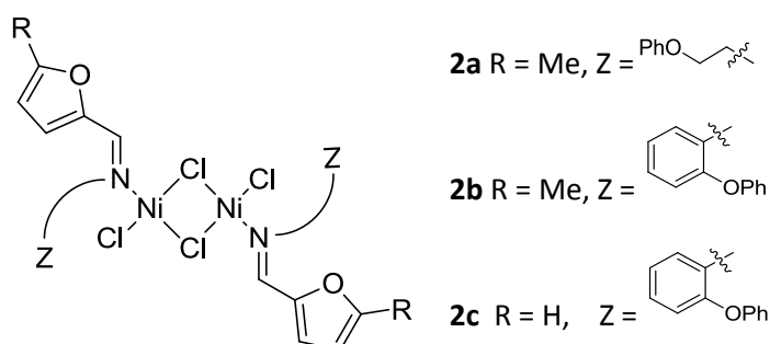
Figure 5. Ether-functionalized imino-furfural complexes
