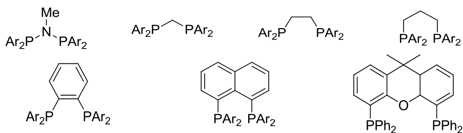
Figure 13. Different (P,P)-bidentate ligands developed by Wass et al. 11
