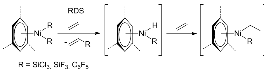
Scheme 15. Ni-H formation from [\text{Ni}(\eta^6\text{-arene})\text{R}_2]
