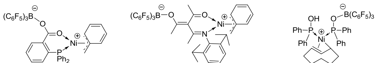
Figure 51. Zwitterionic (P,O)-based isolated active complexes
