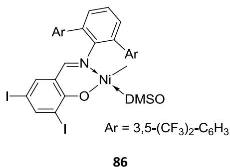
Figure 53 : Cationic methylnickel complex synthesized by Berkefeld and Mecking
