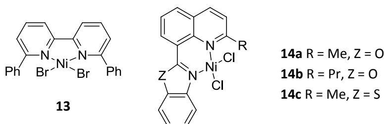
Figure 11. Imino-bis-heterocyclic-based nickel(II) complexes
