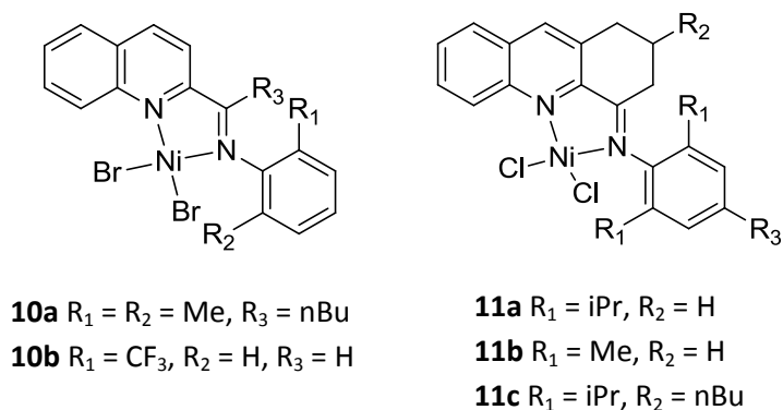
Figure 9. Iminoquinoline based nickel(II) complexes
