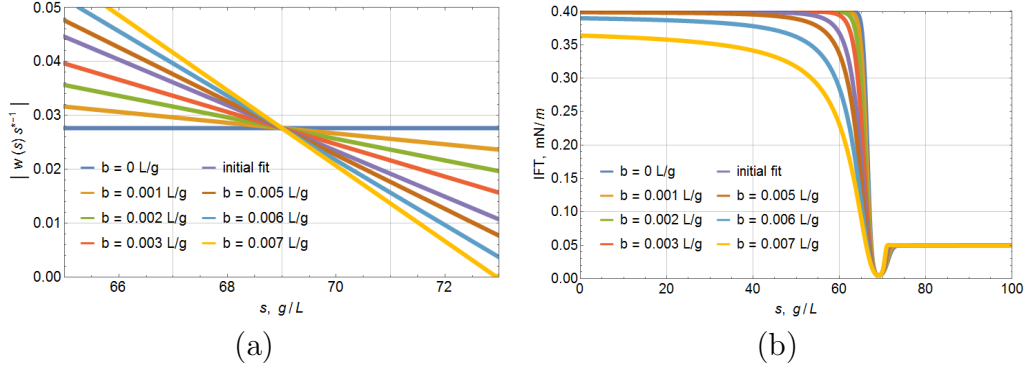
Figure 9: (a) Studied variations of the salinity window w(s)s^{*-1} (9) and (b) the corresponding IFT (7, 8) calculated for the surfactant concentration c = 3 g/L.
