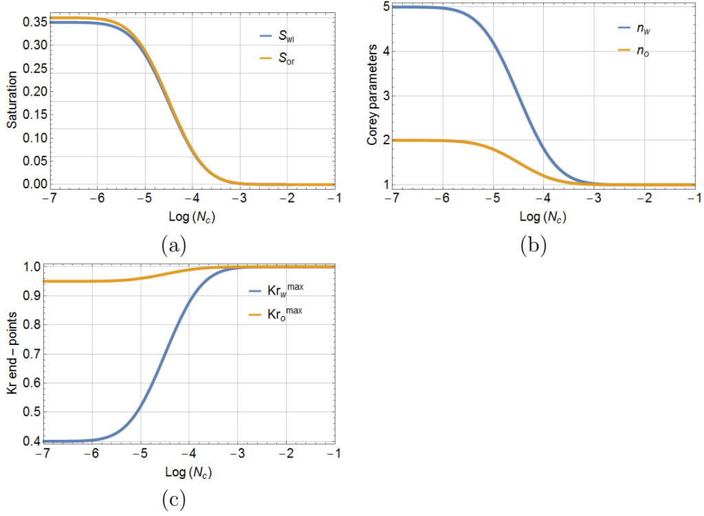
Figure 10: The end-points (Table 6) dependence on the capillary number N_c given in [26, 27].
