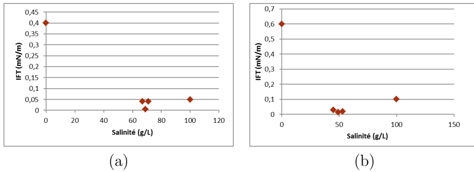
Figure 5: IFT measurements with spinning drop tensiometer versus salinity at 20°C (a) and 40°C (b).
