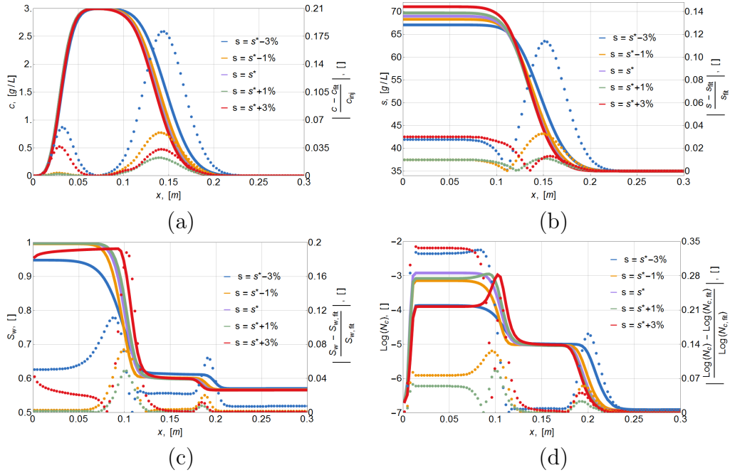
Figure 14: The surfactant concentration (a), salinity (b), water saturation (c) and capillary number (d) in the core at \approx 4 IPV). The dots (right-hand axis labels) correspond to the relative difference between the results for various s_{inj} and those obtained for s_{inj} = s^* .
