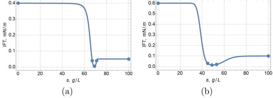
Figure 6: IFT correlation as function of salinity for 20°C (a) and 40°C (b).
