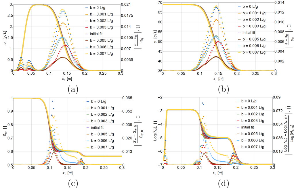
Figure 11: The resulting surfactant concentration (a), salinity (b), water saturation (c) and capillary number (d) in the core at time \approx 0.054 days \approx 4 injected pore volumes (IPV). The dots (right-hand axis labels) correspond to the relative difference between the results for various b and those obtained using its fitted value.
