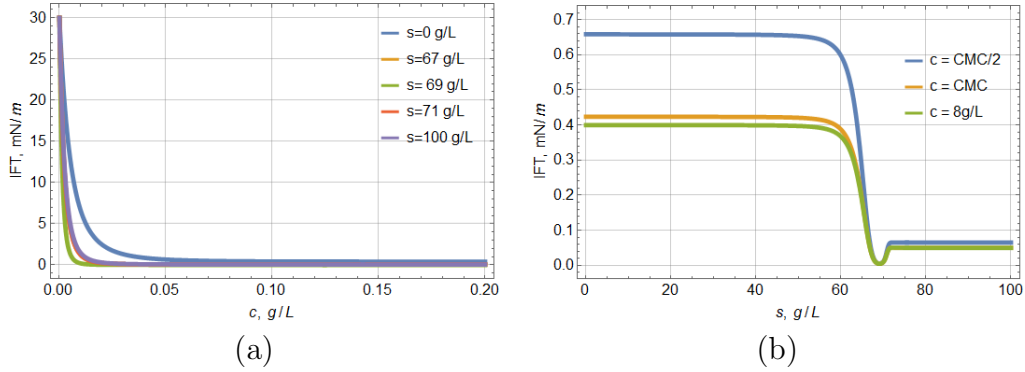
Figure 8: IFT as function of surfactant concentration for a few salinity values (a) and as function of salinity for a few fixed values of the surfactant concentration within the "transition" range and far from CMC.
