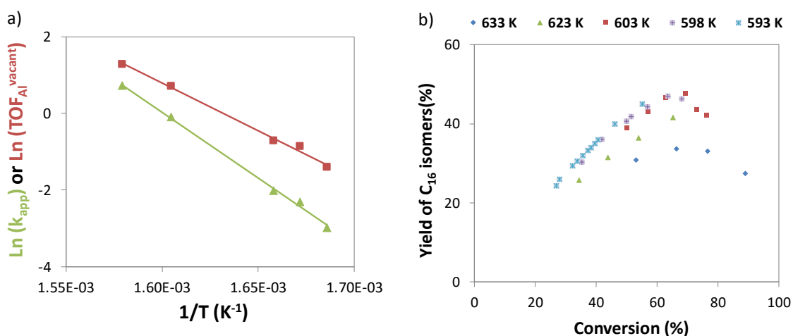
Figure 2: a) Arrhenius' plot for catalytic activity ( \blacktriangle ) and turnover frequency per available protonic site ( \blacksquare ). Symbols stand for experimental data and lines for model fitted Arrhenius' equation. Units of k_{\text{app}} : \mu\text{mol g}_{\text{zeolite}}^{-1} \text{s}^{-1} . Units of \text{TOF}_{\text{Al}}^{\text{vacant}} : \text{s}^{-1} (molar basis). b) Yield of feed isomers as function of conversion at different reaction temperatures. Catalyst: \text{NiMoS}/(\text{Al}_2\text{O}_3+\text{HUSY}) .
