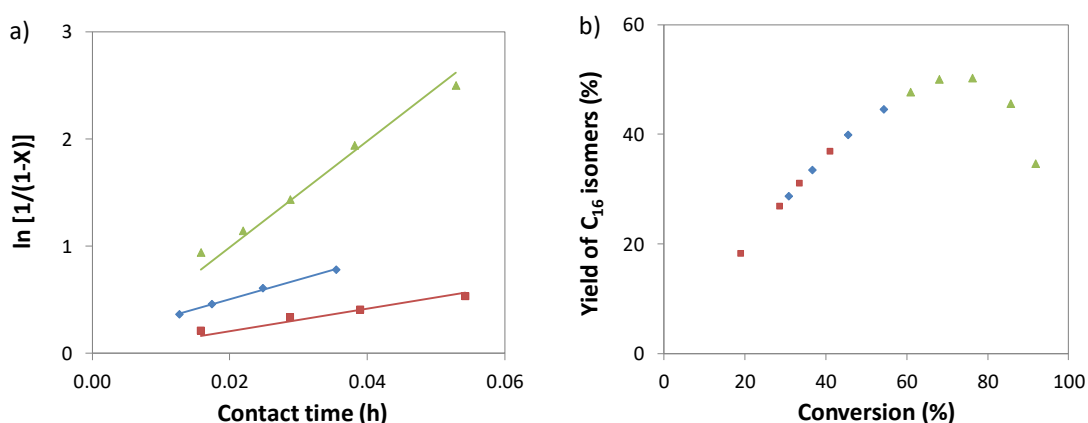
13 Figure 1: a) 1 st -order plot of n -hexadecane conversion (X) as function of contact time and b) 14 yield of C 16 isomers as function of conversion, over Pt/HUSY catalyst. Reaction temperatures: 15 528 (■), 538 (◆), and 548 K (▲). Symbols stand for experimental data and lines for the 16 corresponding linear regression.
