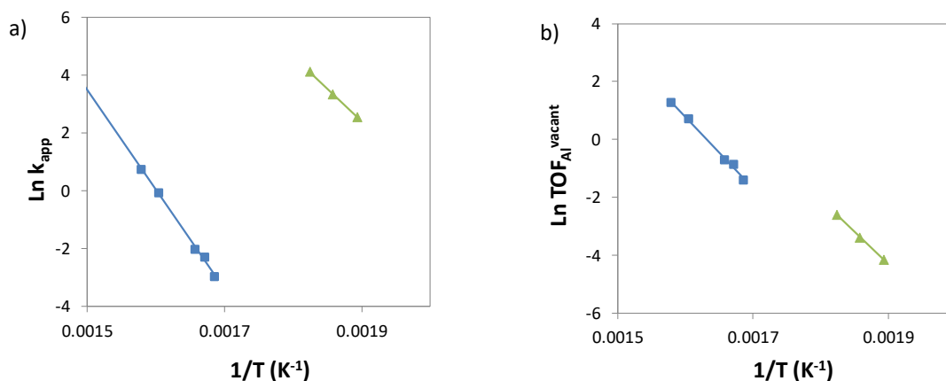
Figure 4: Arrhenius's plot for a) catalytic activity and b) turnover frequency per vacant protonic site over Pt/HUSY (▲) and NiMoS/(Al 2 O 3 +HUSY) (■) catalysts. Symbols stand for experimental data and lines for regression of the Arrhenius equation. Units of k_{app} : \mu\text{mol g}_{zeolite}^{-1} \text{s}^{-1} . Units of TOF_{Al}^{vacant} : \text{s}^{-1} (molar basis).
