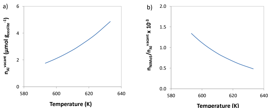
Figure 3: Estimated evolution of a) the concentration of vacant acid sites in the HUSY zeolite and b) the molar ratio of NiMoS to vacant Brønsted sites with temperature, under reaction conditions.
