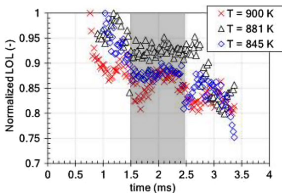
Fig. 13. Time evolution of the normalized Lift-Off Length (LOL) at different ambient temperatures: experiments performed in PPRIME-RCM , each temperature case is an average of three tests.
