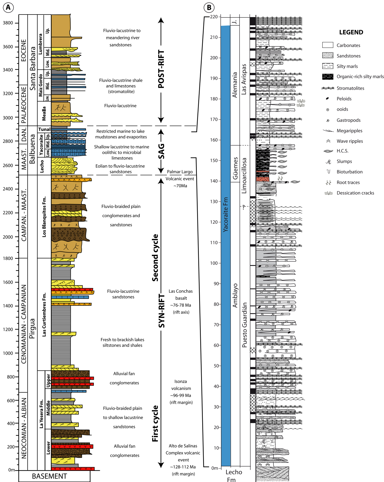
FIGURE 3 Stratigraphic section of the sedimentary fill from the Salta rift basin based on outcrop observation (modified from Marquillas et al. , 2005). To the left: Cabra Corral/Juramento area synthetic section
