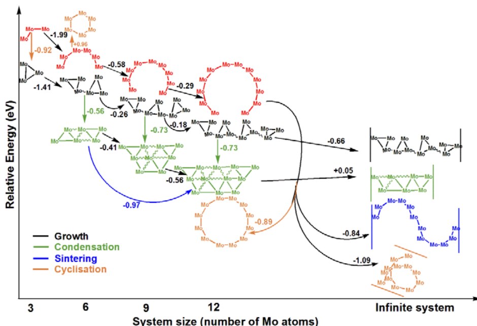
Figure 6: Possible transformation pathways of the MoS 3 polymorphs and correspondingly free energy change.
