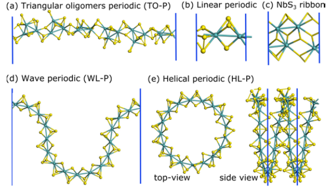
Figure 2 : Various \text{MoS}_3 nanostructures : a) Triangular oligomers \text{Mo}_{18}\text{S}_{54} (TO-P), (b) Linear periodic \text{Mo}_2\text{S}_6 (L-P), (c) \text{NbS}_3 -ribbon ( \text{Mo}_4\text{S}_{12} ) (d) \text{Mo}_{16}\text{S}_{48} Wave-like (WL-P), and (e) \text{Mo}_{17}\text{S}_{51} Helical (HL-P). Direction perpendicular to the blue lines is the direction of periodicity.
