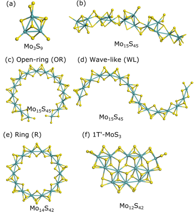
Figure 1 (a) Various oD- MoS_3 nano-structures: Triangular monomer Mo_3S_9 and triangular oligomers (TO) Mo_{15}S_{45} , (c) open ring (OR) conformer, (d) Wave like (WL), (e) Ring (R) and (f) 1T' - MoS_3 (see text for explanation).
