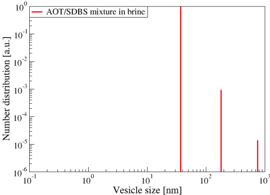
Figure 5 : Number distribution of vesicles in the AOT (0.16 g/L) / SDBS (0.032 g/L) mixture solution (3.6CVC M )
