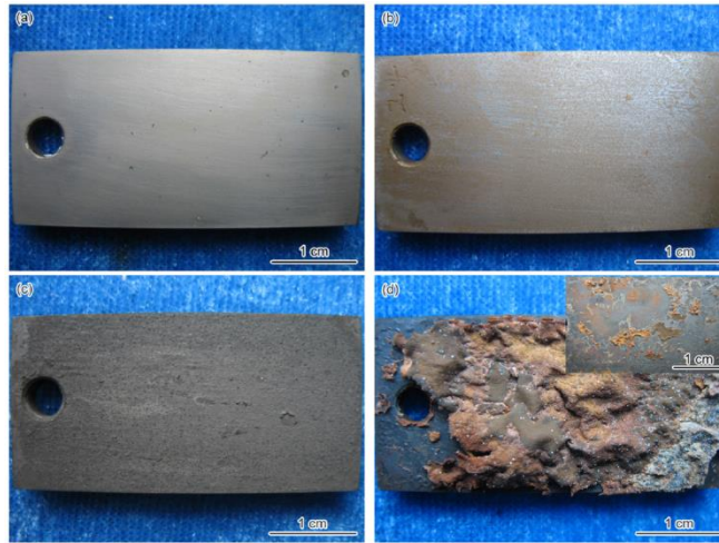
Figure 7 Photographs of corrosion product layer developed at 50°C CO 2 : 10 MPa, O 2 : 2000 ppmv, H 2 S: 2000 ppmv. (a) CO 2 ; (b) CO 2 + O 2 ; (c) CO 2 + H 2 S and (d) CO 2 + O 2 + H 2 S [77].
