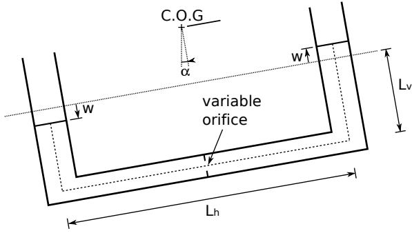
Fig. 1. Scheme of the TLCDF in motion.
