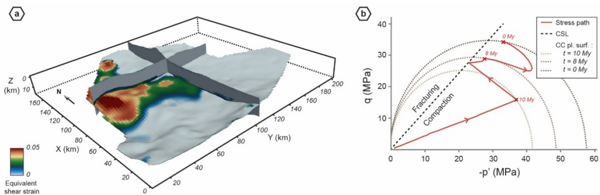
Figure 12 – Natural fracturing of the Vaca-Muerta Fm in the coupled simulation. (a) 3D view of the model showing the distribution of the cumulated von Mises strain, or fracturing. Vertical exaggeration is set to x5. (b) Stress path of a cell from the base layer of the Vaca-Muerta Fm, in a (p';q) diagram. The CamClay yield surfaces are computed for three key events of the simulation.
